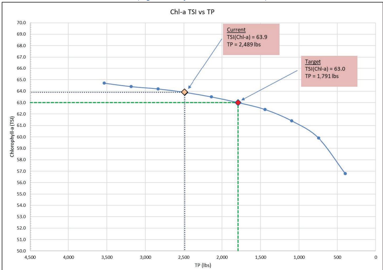
Figure 1 Simulated Load Response between Chlorophyll-a Trophic State Index and Total Phosphorus Load (Figure 3-8 of the TMDL document)
