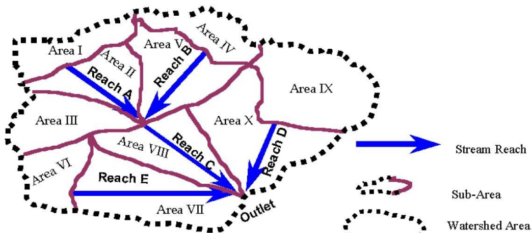
Figure C3-S5-6: Sample watershed schematic for WinTR-55
