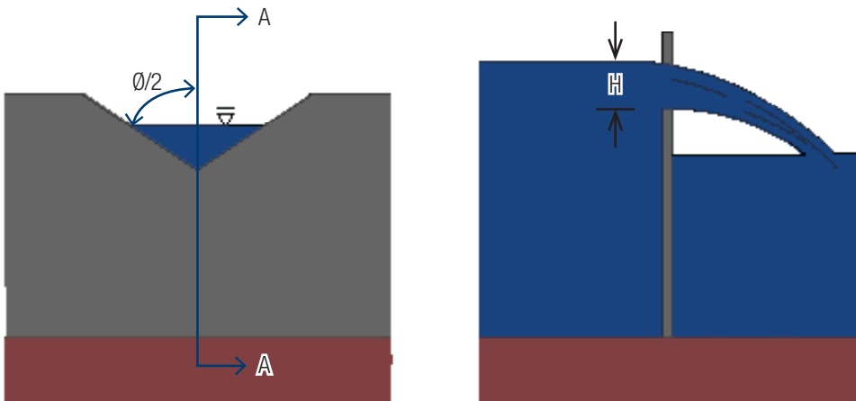
Figure 9.04-3.4: Variable illustration for V-notch weirs
