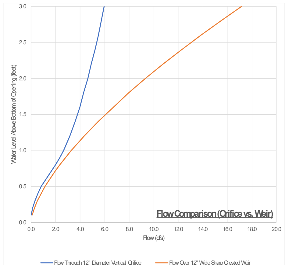
Figure 9.04-3.1: Graph comparison of flow across a weir vs. head condition
