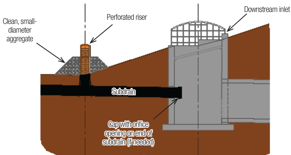
Figure 9.04-2.2: Example Perforated Riser arrangement
