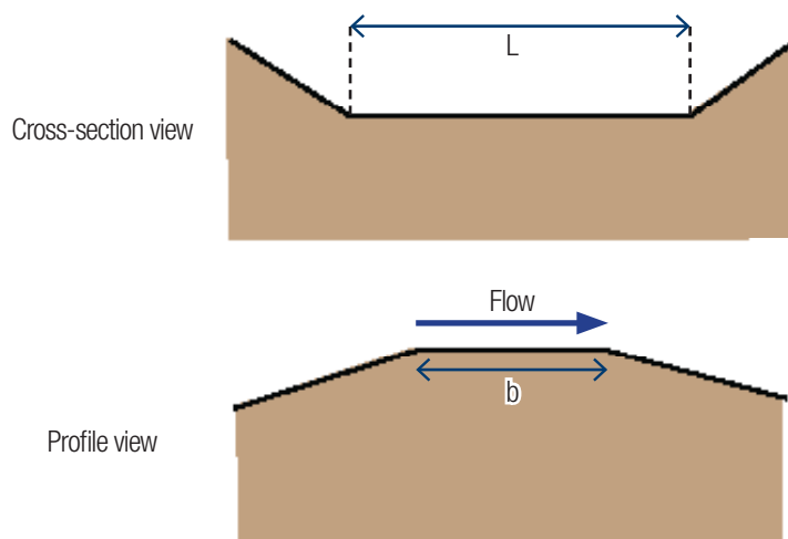
Figure 9.04-3.3: Side, cross-section illustrations of a broad-crested weir
