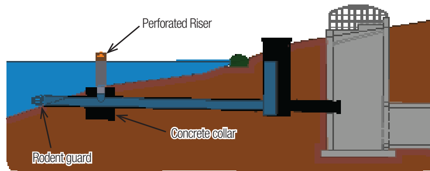
Figure 9.04-6.4: Subsurface inlet protections
