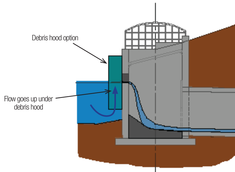
Figure 9.04-6.1: Subsurface inlet using debris hood
