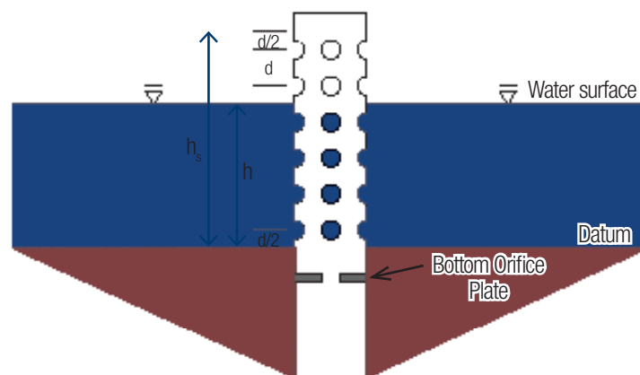
Figure 9.04-2.1: Perforated riser variable definitions. (1)
