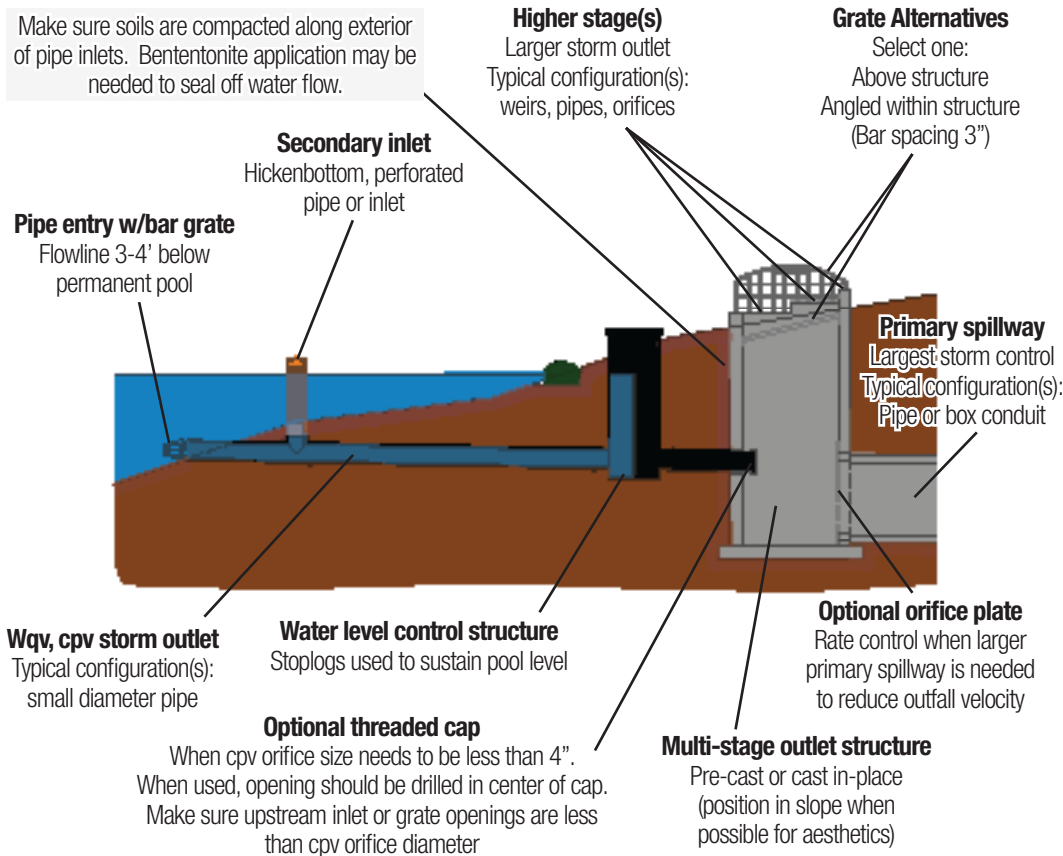
Figure 9.04-5.1: Multi-stage outlet example
