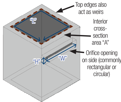
Figure 9.04-5.2: Example of a Multi-stage Outlet with Weirs on Top and Orifice on Side
