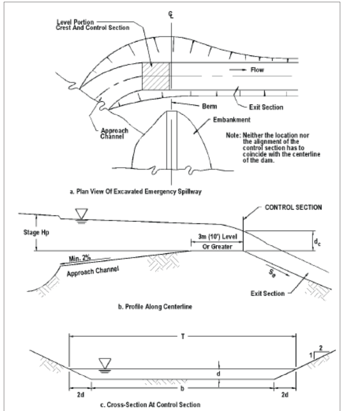
Figure 9.04-8.1: Auxiliary Spillway Design Schematic (5)
