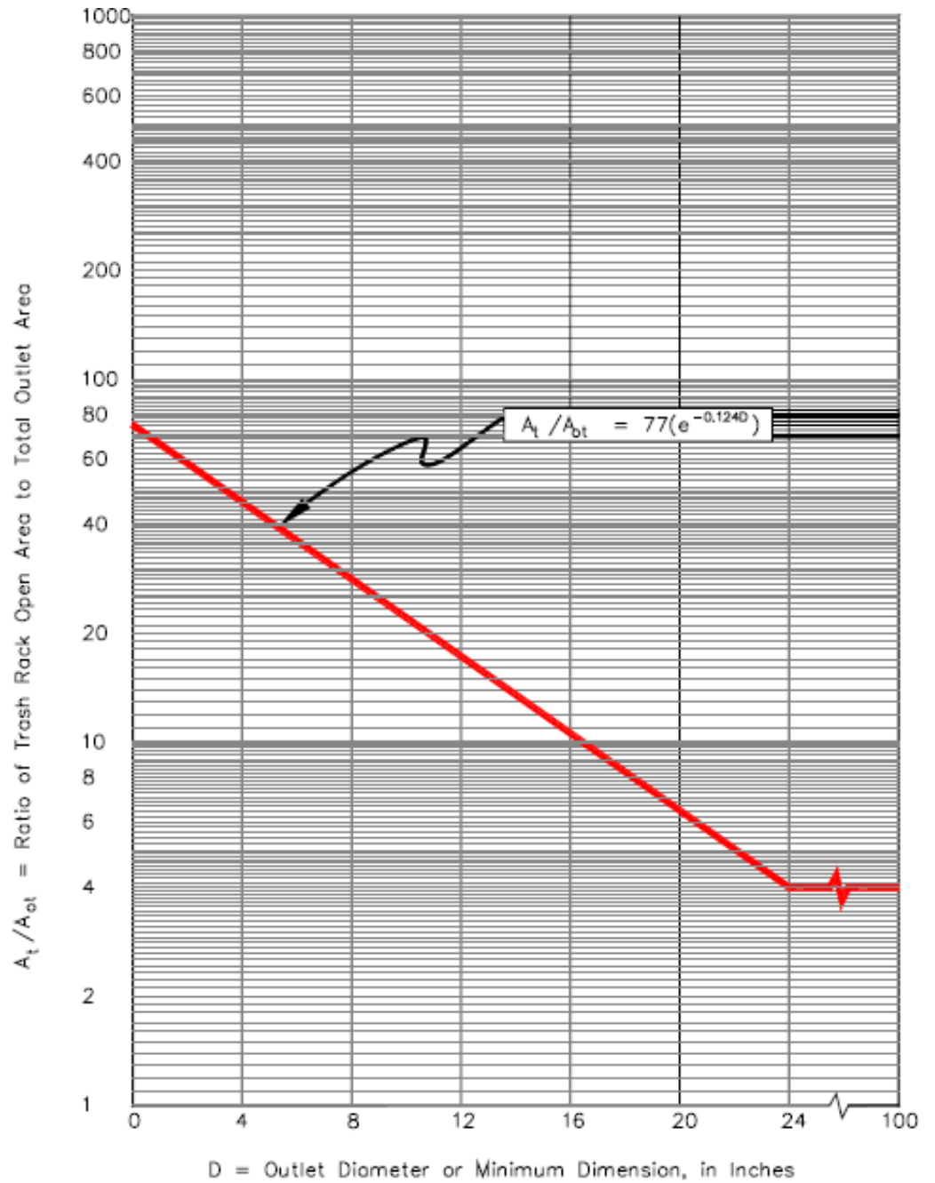
Figure 9.04-7-2. Minimum trash rack open area
