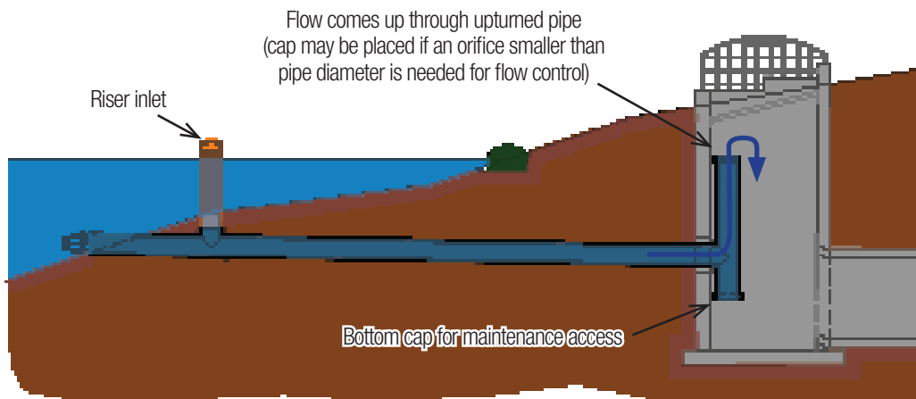
Figure 9.04-6.3: Upturned Riser example
