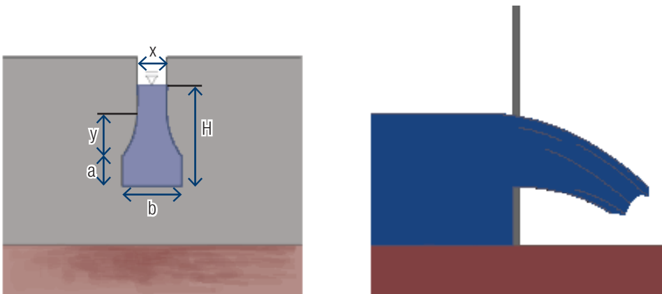
Figure 9.04-3.6: Proportional Weir Dimensions
