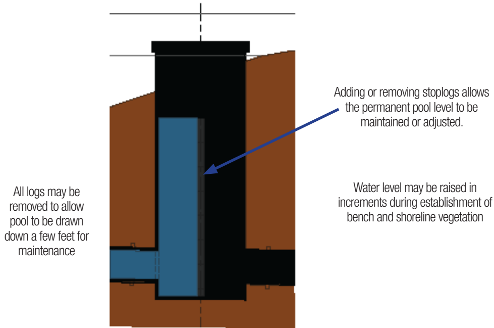
Figure 9.04-6.2: Water Level Control Structure
