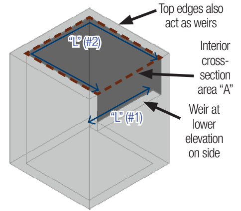
Figure 9.04-5.3: Example of a Multi-stage Outlet with Weirs on Top and Lower Weir on Side
