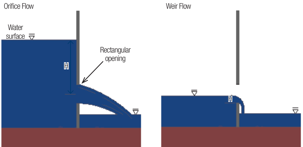
Figure 9.04-5.4: Illustration of transition between orifice and weir flow conditions through an opening
