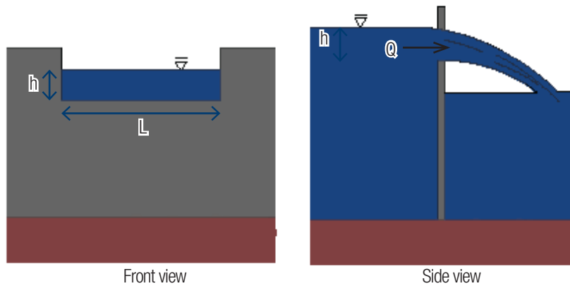
Figure 9.04-3.2: Rectangular Weirs
