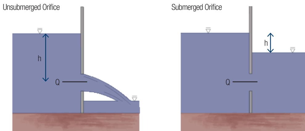
Figure 9.04-2.3: Measurement of Head Conditions for Unsubmerged and Submerged Orifices
