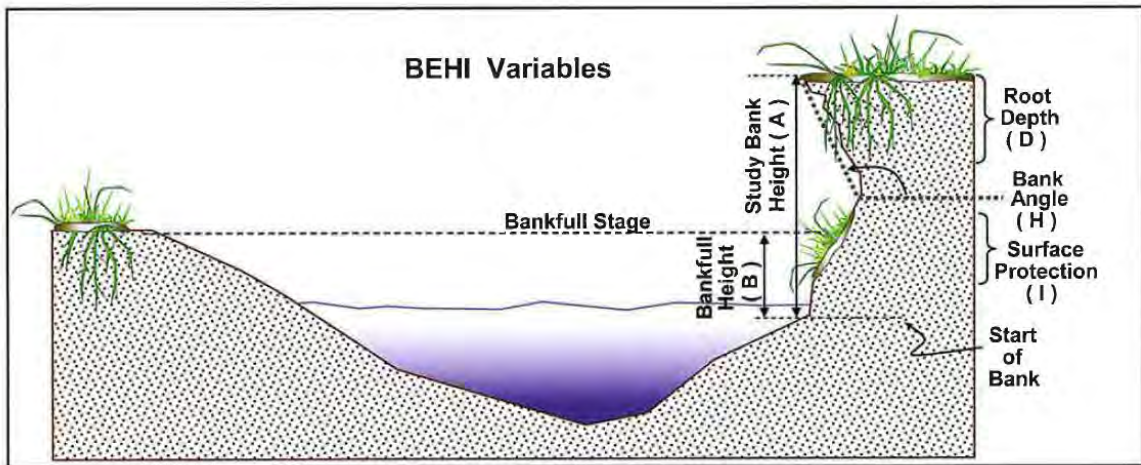
Figure 5-14. Diagram depicting the BEHI variables.
