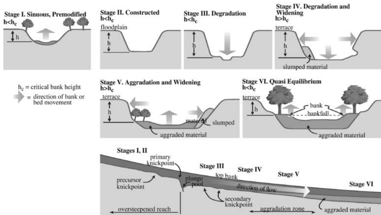
Channel Evolution Model (Schumm and Parker 1973) modified (Simon and Rinaldi, 2006)
