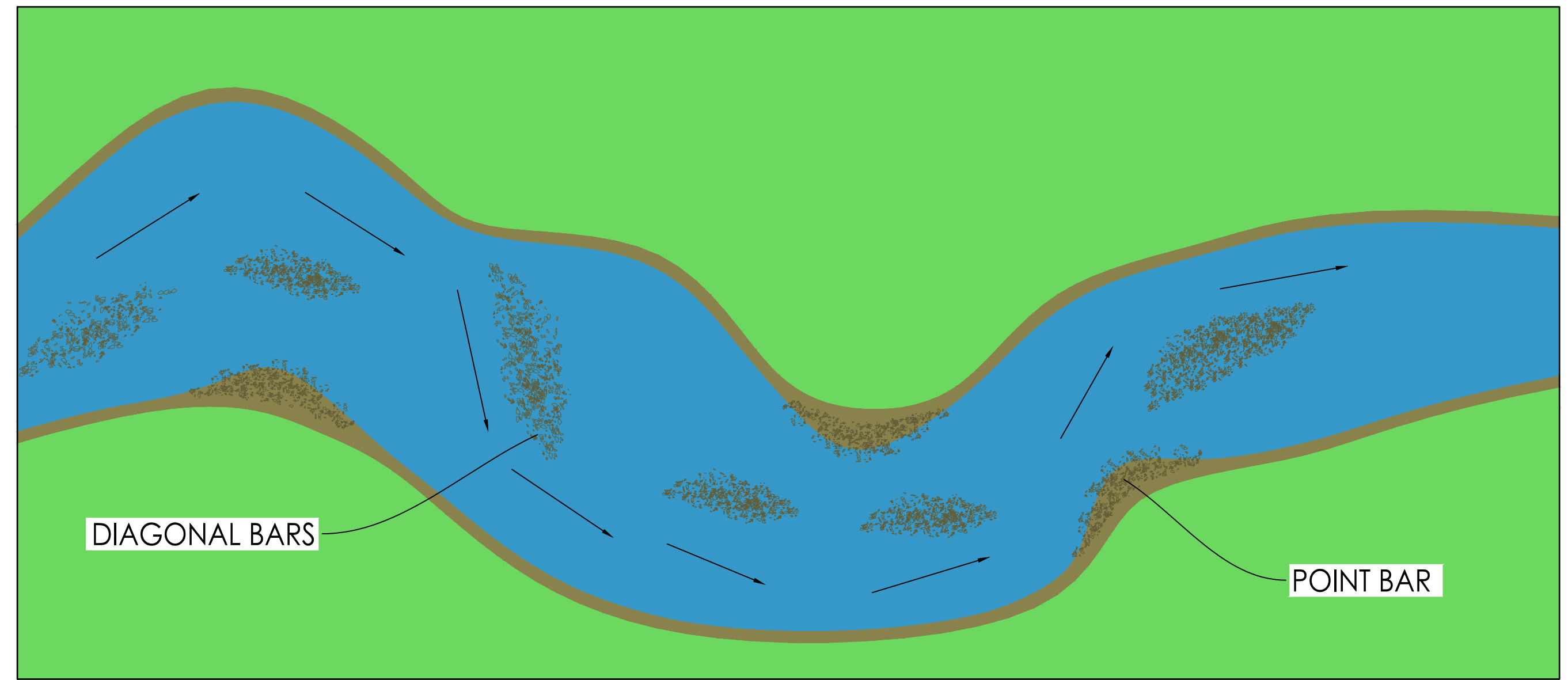
DIAGONAL BARS
