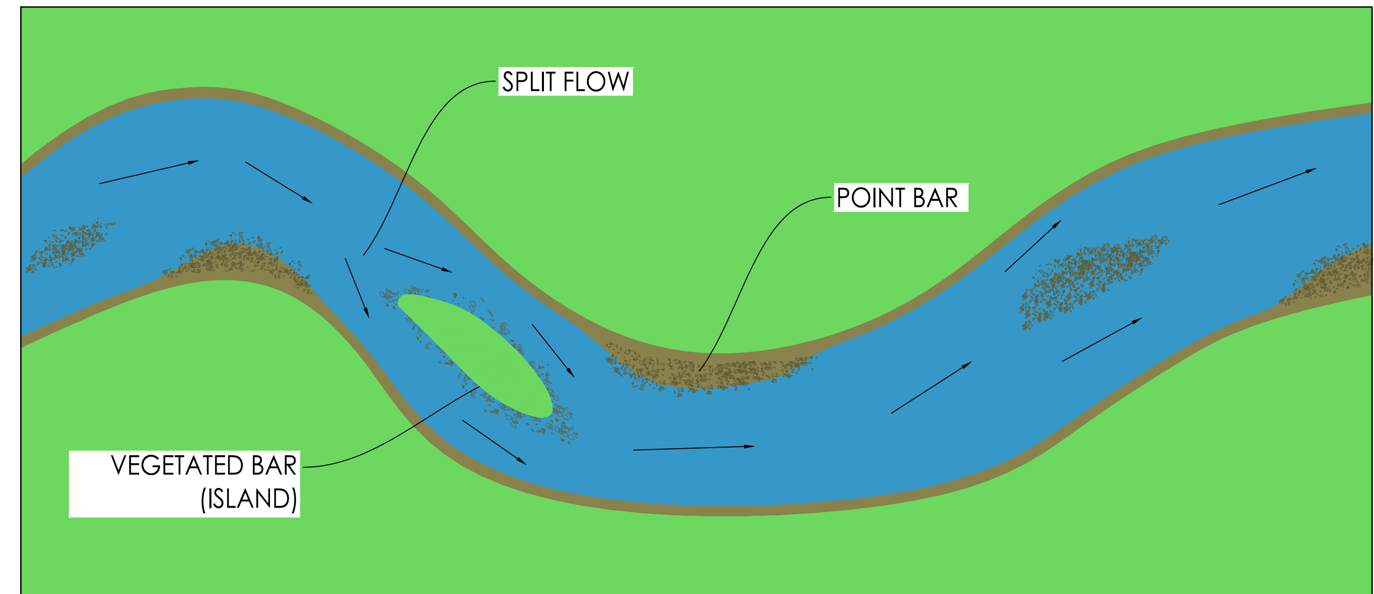
SPLIT FLOW
