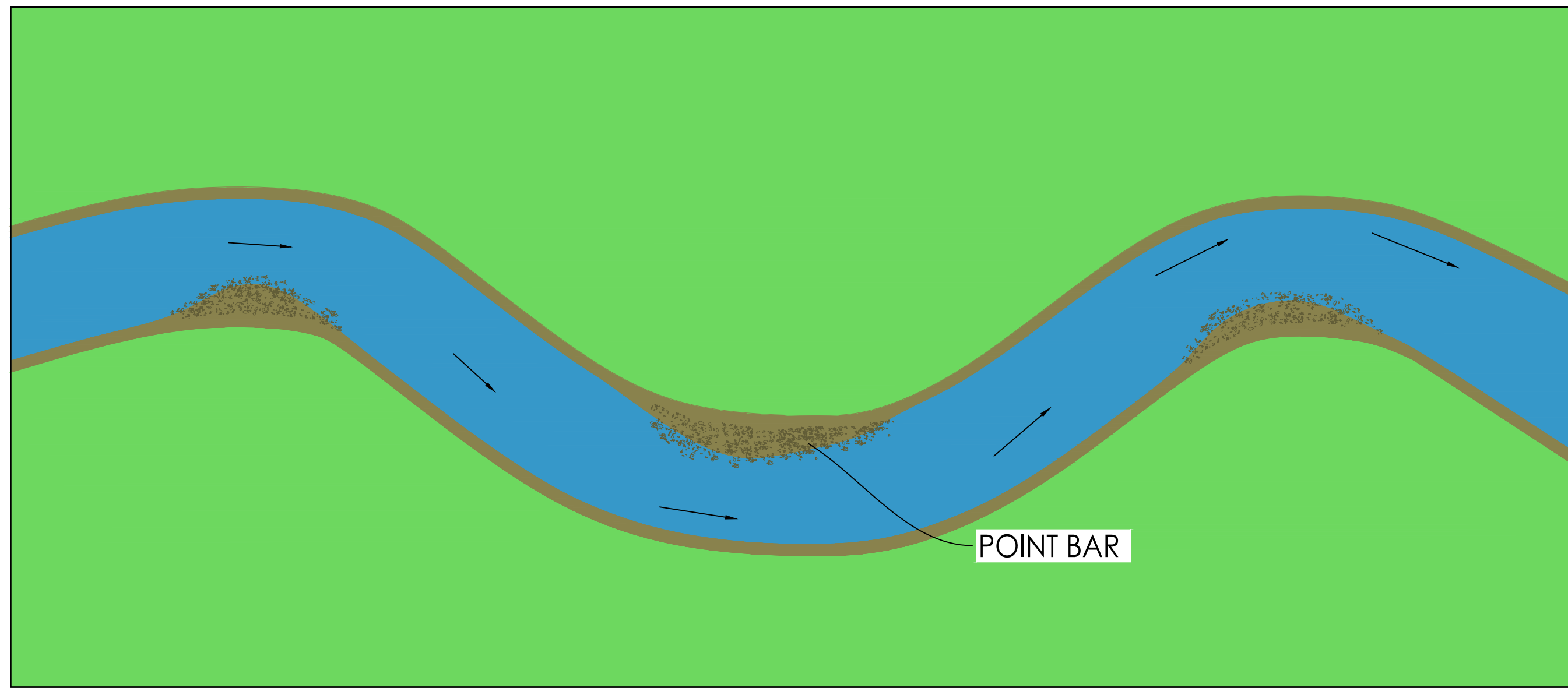
POINT BARS
