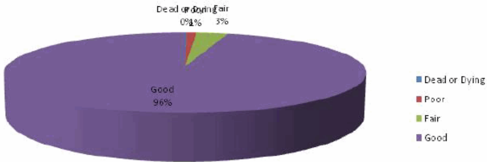
Figure 3: Foliage Condition
