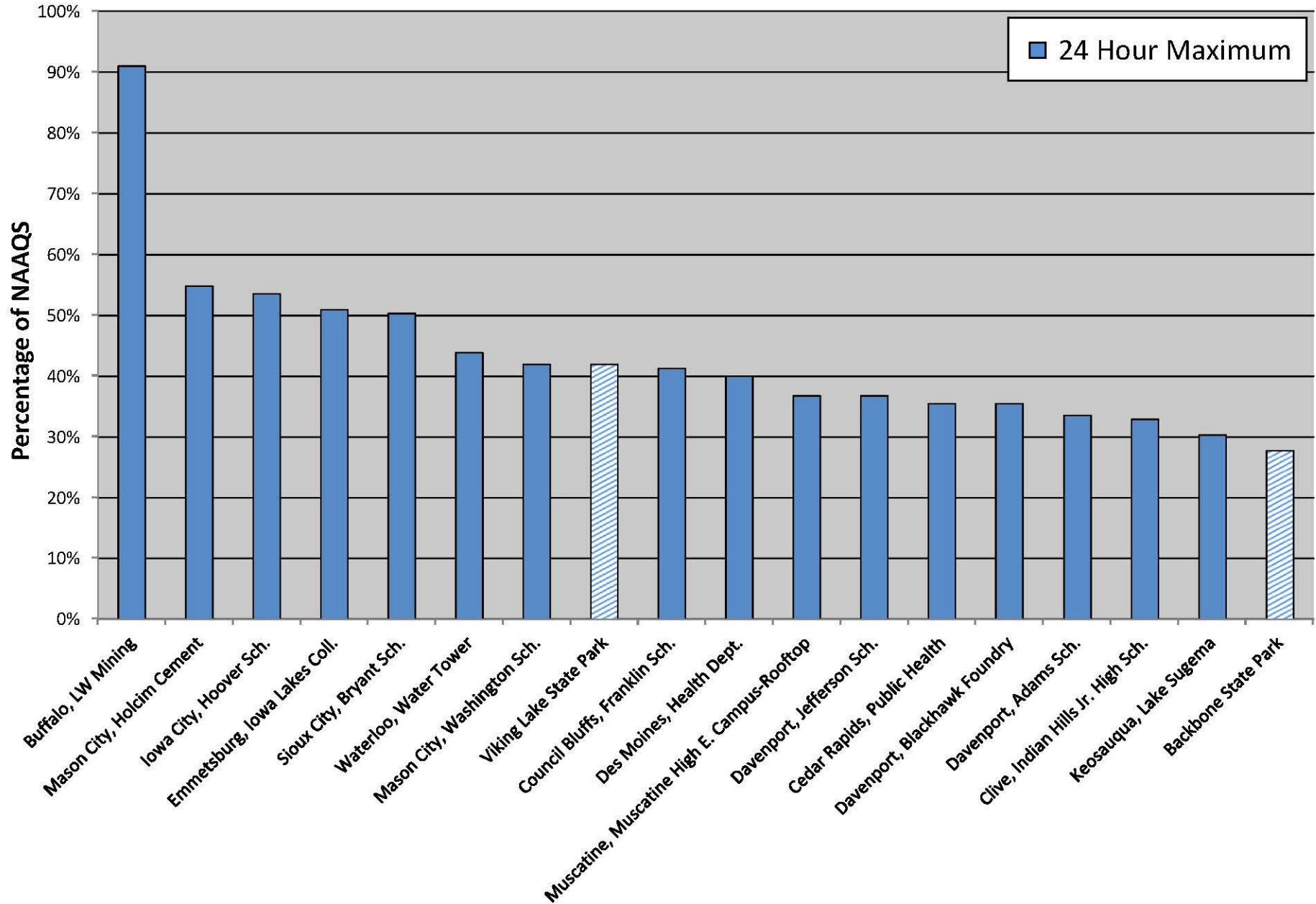
Comparison of 2012 PM 10 Data with the National Ambient Air Quality Standard
