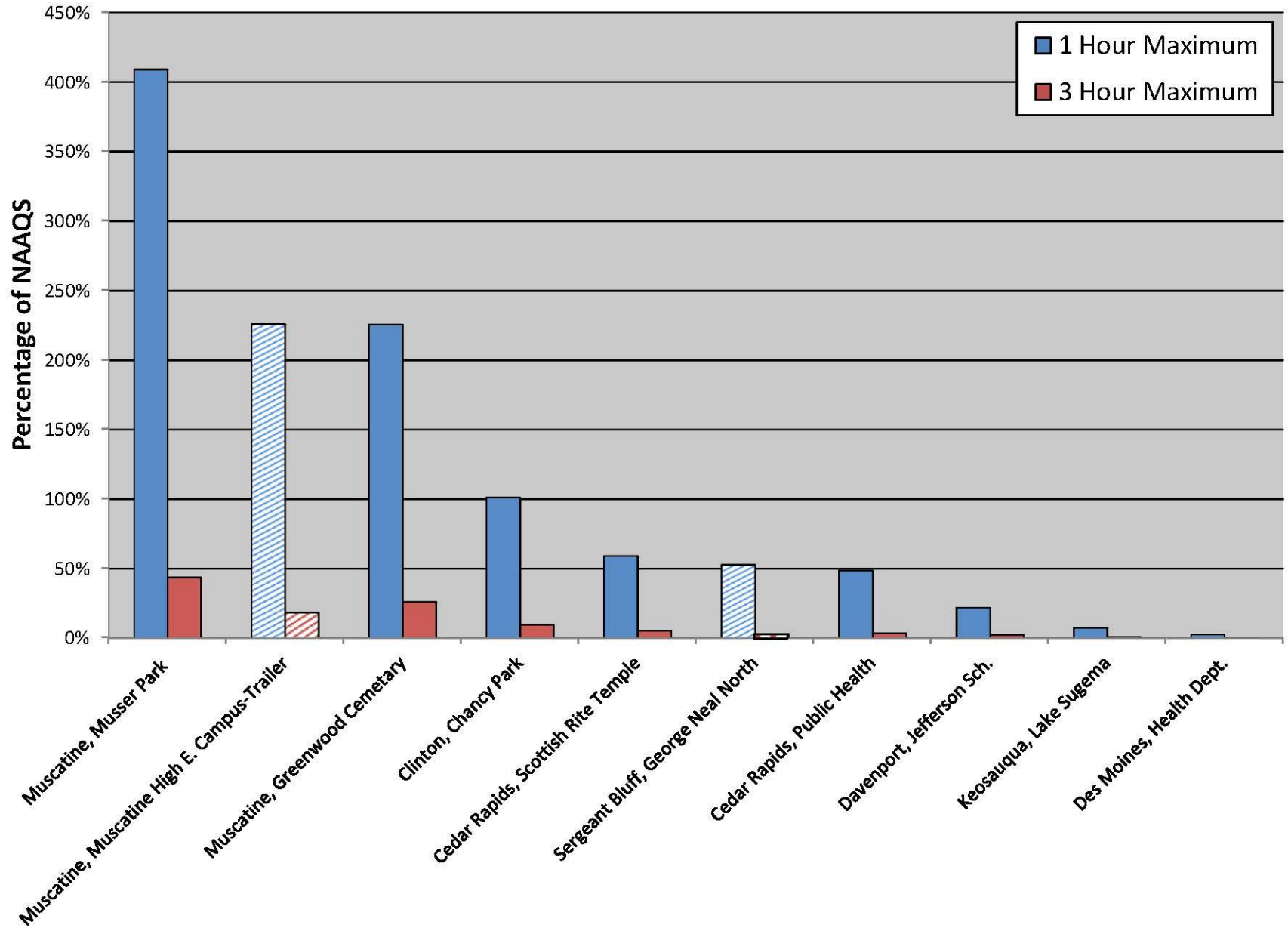
Comparison of 2012 Sulfur Dioxide Data with National Ambient Air Quality Standards
