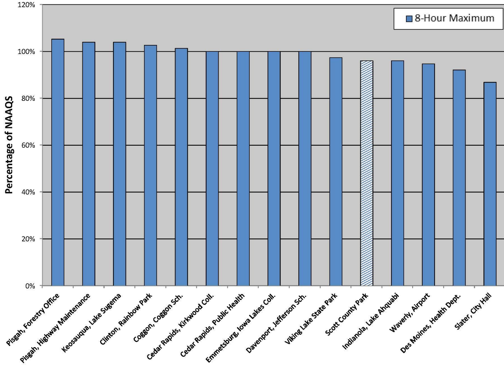
Comparison of 2012 Ozone Data with National Ambient Air Quality Standards
