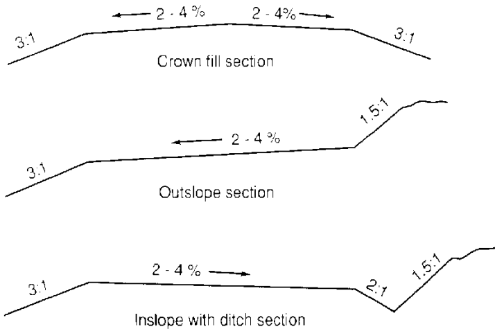
Figure C-6. Typical road designs form drainage and stability. (Adapted from Wisconsin Department of Natural Resources, 1995.)
