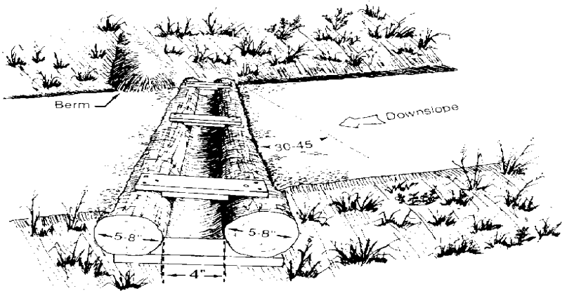
Figure C-8. Open-top log culvert. (Adapted from Wisconsin Department of Natural Resources, 1995.)
