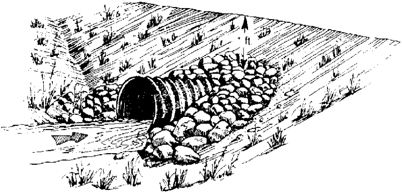
Figure C-5a. Use riprap around the inlet of culverts.
