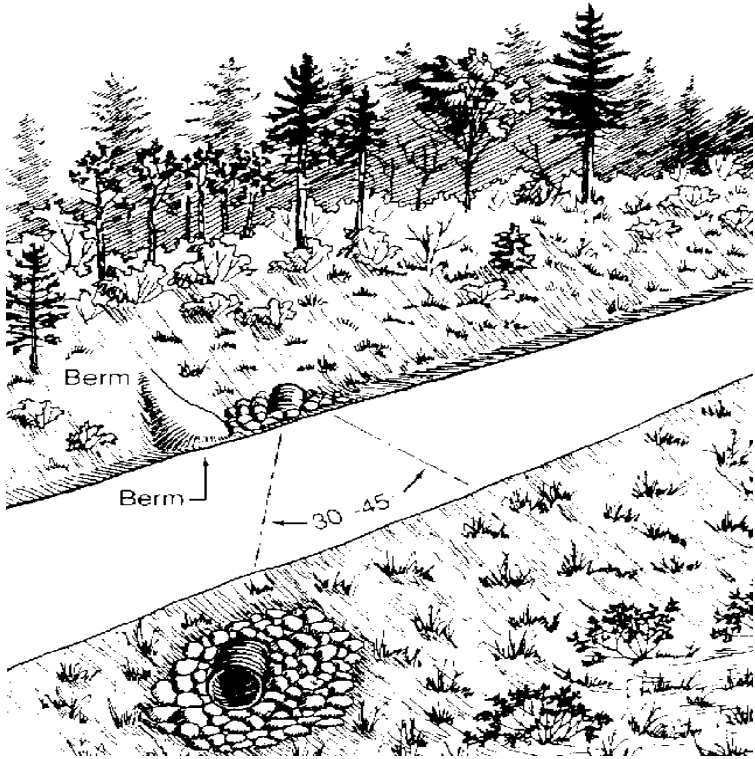
Figure C-7. Cross-drain culvert. (Adapted from Wisconsin Department of Natural Resources, 1995.)
