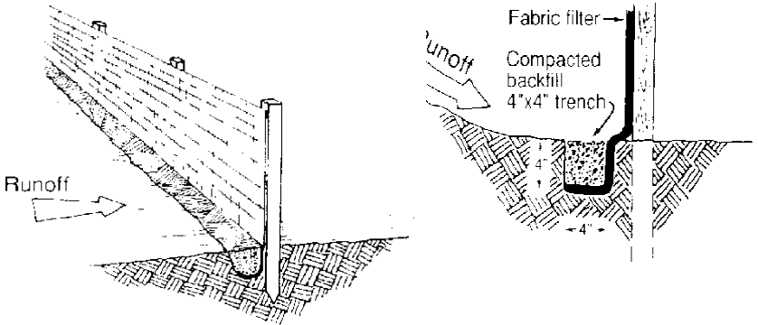
Figure C-11b. Silt fencing to slow runoff and trap sediment for sheet flow, not channelized flow. (Adapted from Wisconsin Department of Natural Resources, 1995.)
