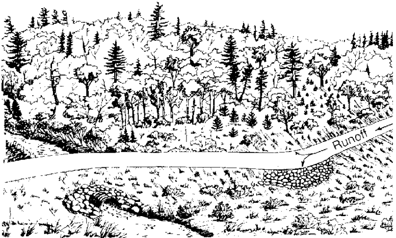
Figure C-1. Place fill directly over a culvert higher than the road approach to prevent surface road runoff from draining onto the crossing structure and into the stream. (Adapted from Wisconsin Department of Natural Resources, 1995.)
