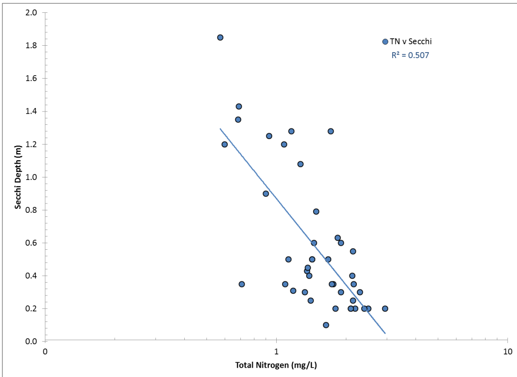
Figure 3-9. Total nitrogen and Secchi depth relationship
