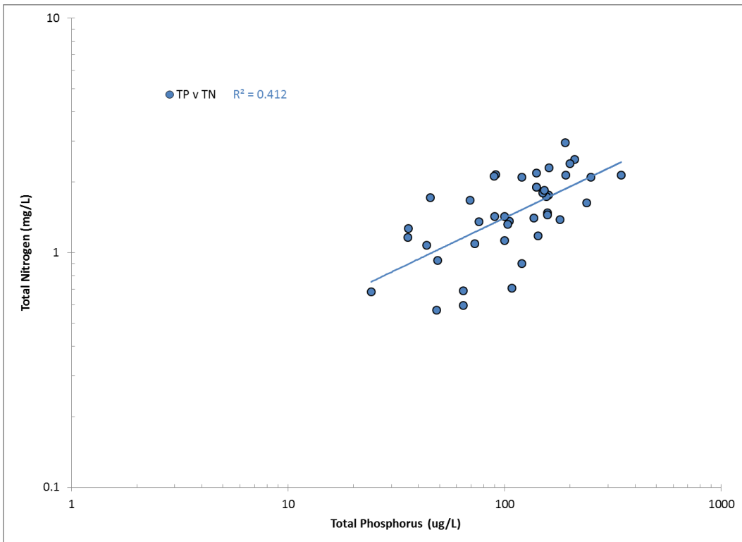
Figure 3-7. Total phosphorus and total nitrogen relationship
