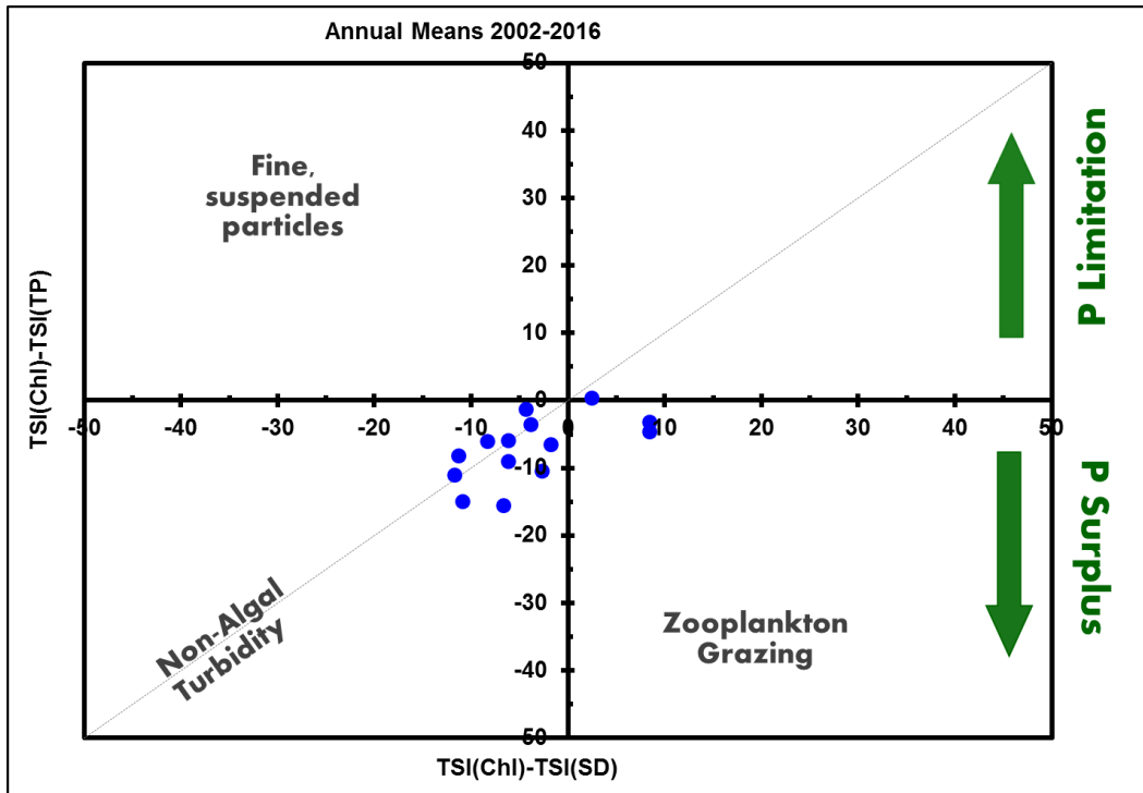
Figure 3-11. Phosphorus TSI deviations annual averages for analysis period
