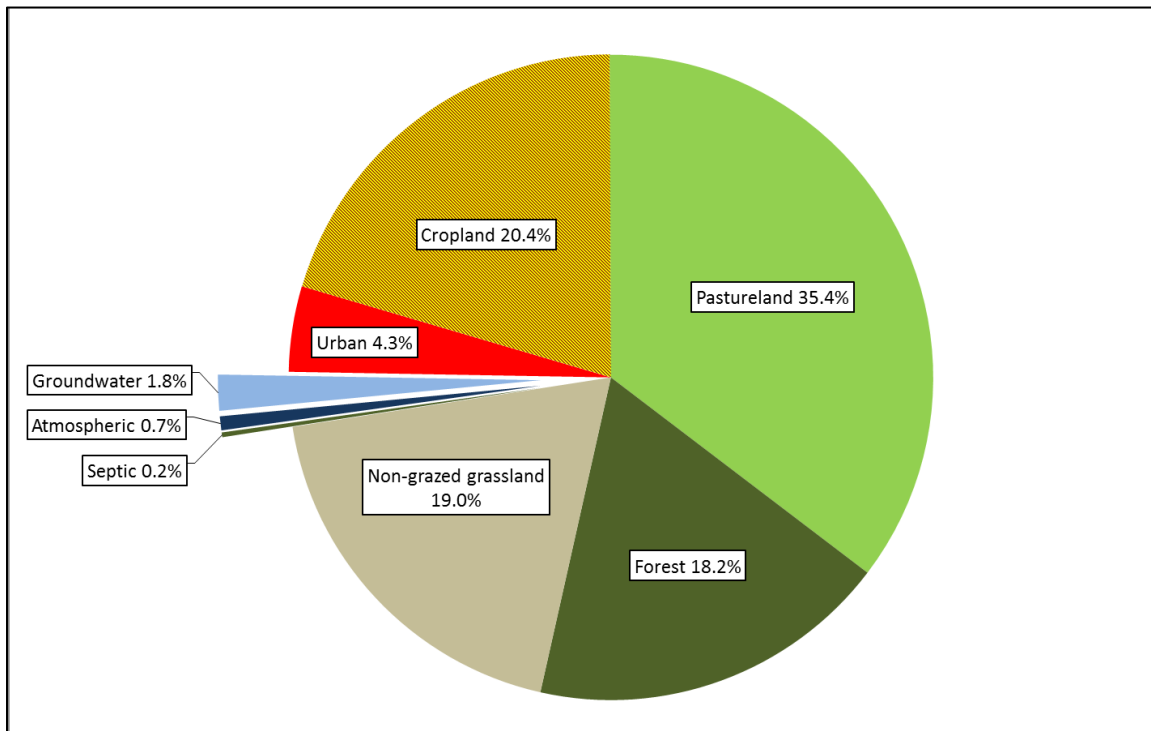
Figure 3-13. Relative TP loads by source
