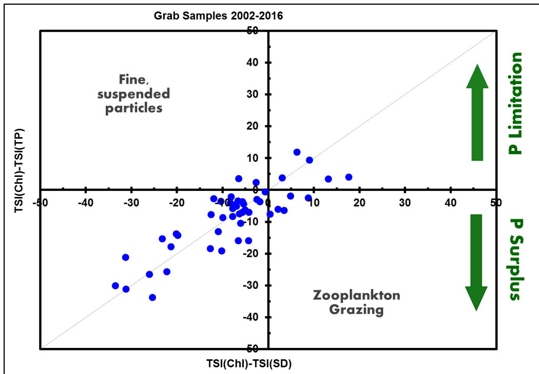
Figure 3-10. Phosphorus TSI deviations grab samples for analysis period
