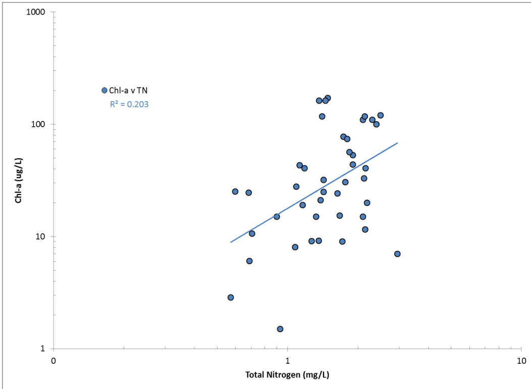
Figure 3-8. Total nitrogen and chl-a relationship
