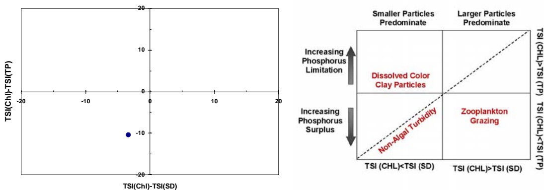
Figure 2. Silver Lake 2000 - 2004 Mean TSI Multivariate Comparison Plot (21)
