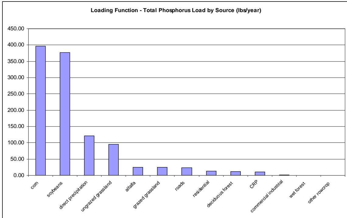
Figure 3. Loading Function Model External Nonpoint Source Contributions
