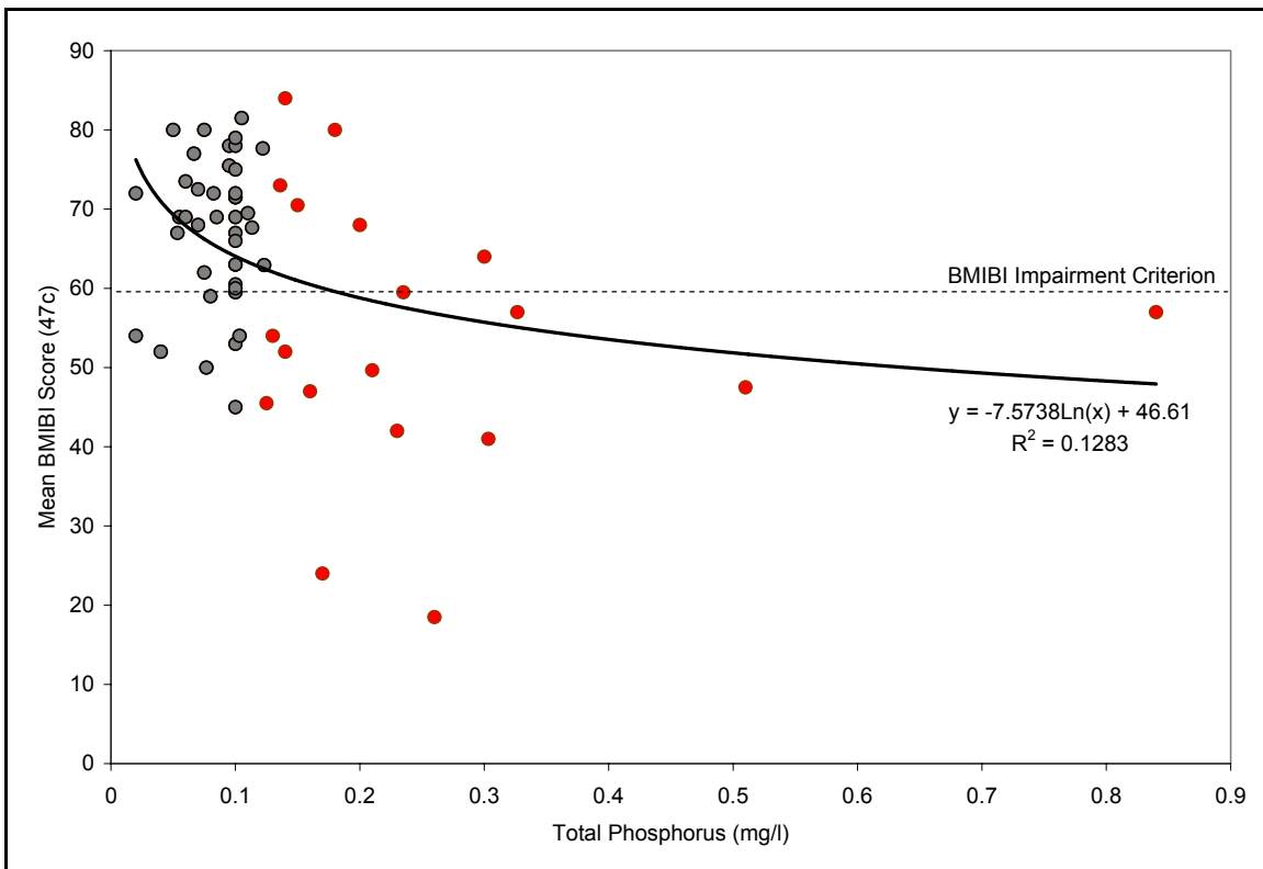
Figure D6. Relationship between TP and BMIBI scores in lowan Surface reference streams. Gray dots represent streams with median TP \leq 0.12 mg/l.
