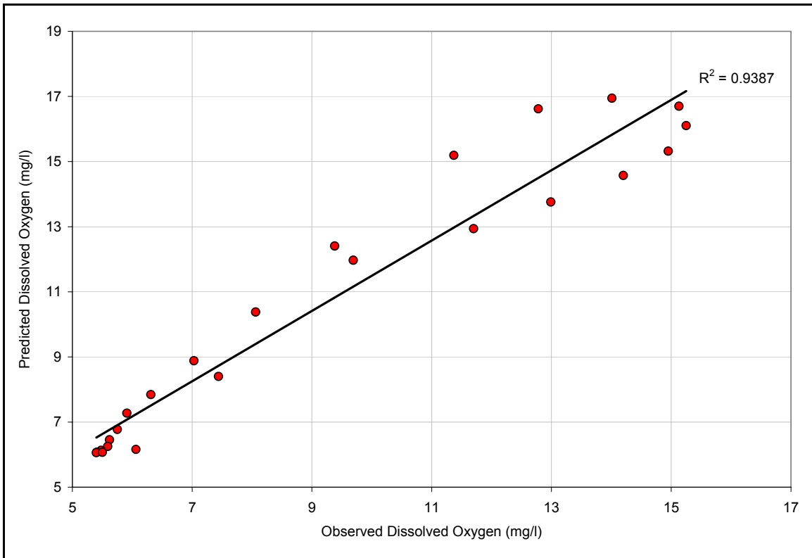
Figure D13. Observed vs. predicted dissolved oxygen values.
