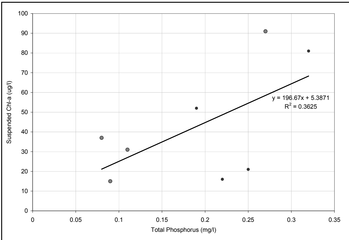
Figure D4. Relationship between TP and suspended chlorophyll-a in two impaired lowland Surface streams. Large circles represent data from Middle Fork S. Beaver Creek.
