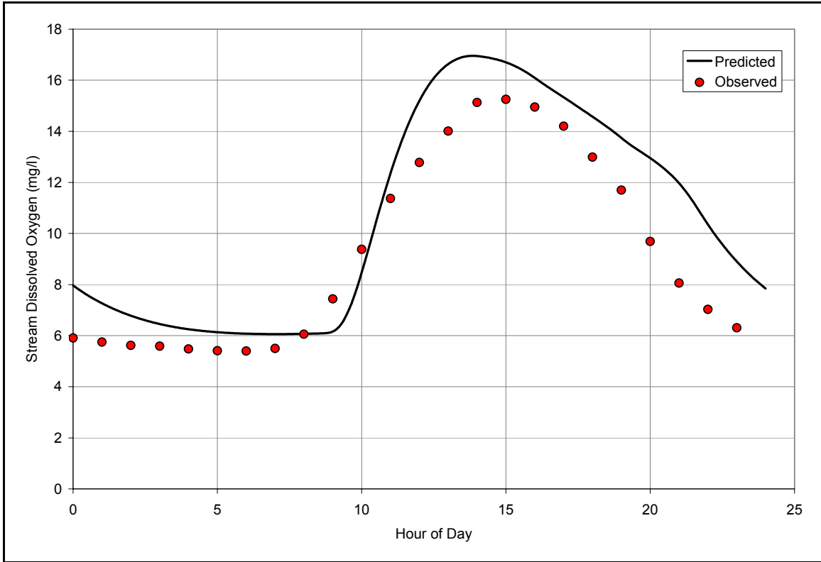
Figure D12. Diurnal dissolved oxygen modeling at downstream site.
