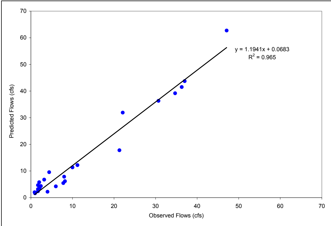
Figure D2. Observed versus predicted flows at the downstream monitoring site.
