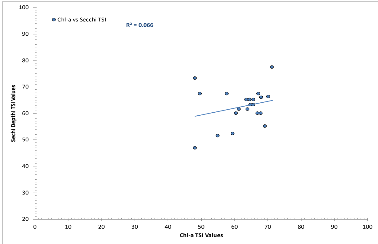
Figure 3-6. Analysis Period TSI Values for Chlorophyll-A and Secchi Depth.
