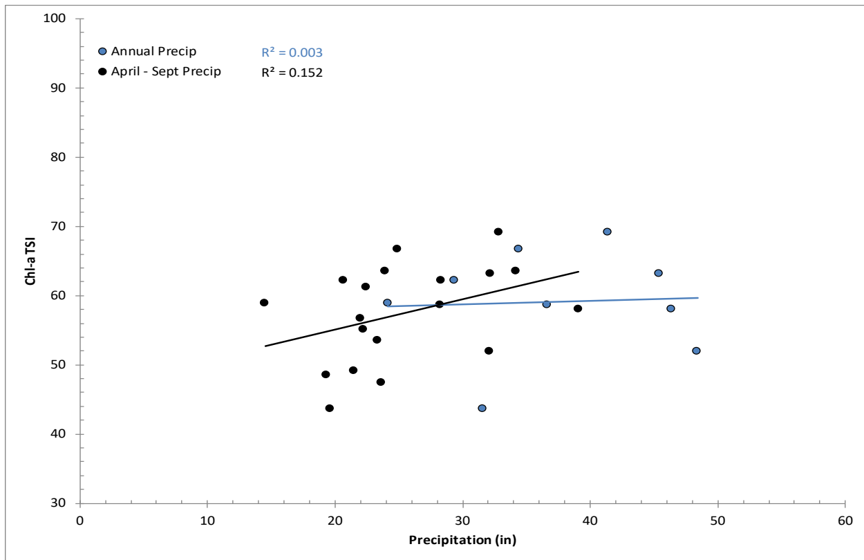
Figure 3-10. Chl-a TSI Values vs Annual and Growing Season Precipitation.
