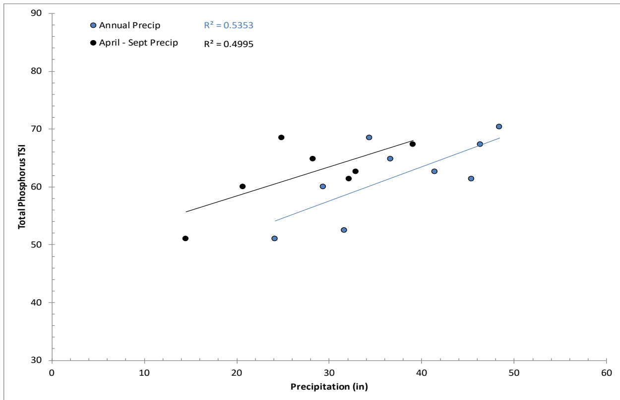
Figure 3-12. Total Phosphorus TSI Values vs Annual and Growing Season Precipitation.
