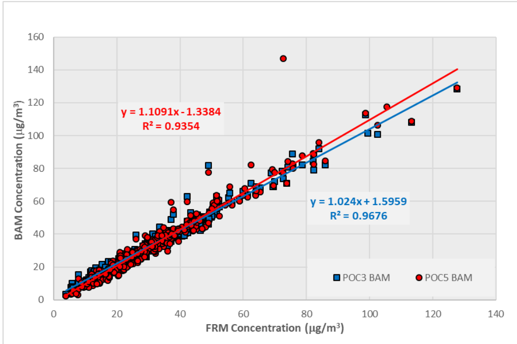
Figure K.3 Buffalo, Linwood Mining PM 10 BAMs vs FRM in 2019
