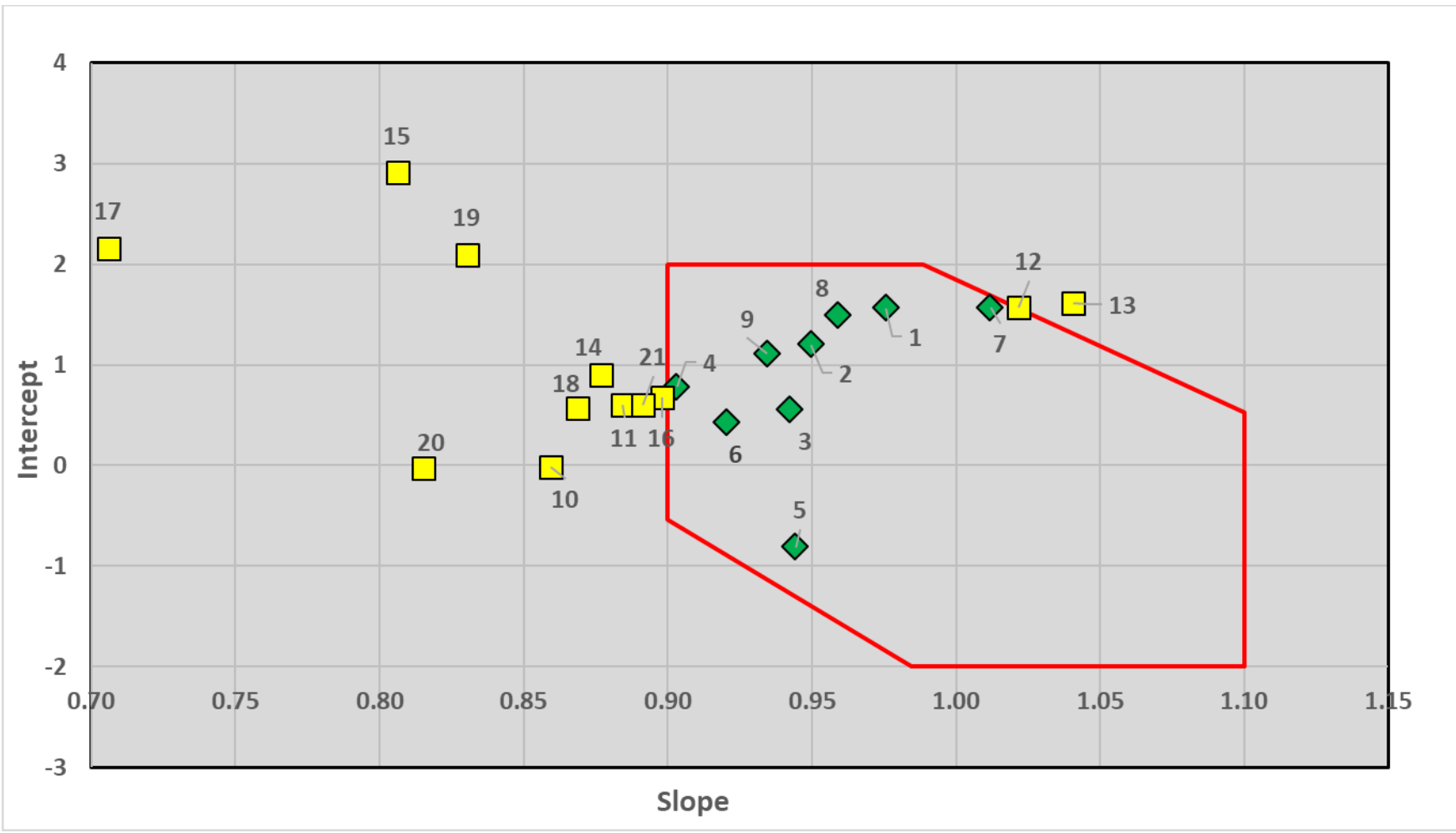
Figure K.2 2019 Continuous PM 2.5 Monitor Performance Relative to the Slope and Intercept Criteria in Part 53.
