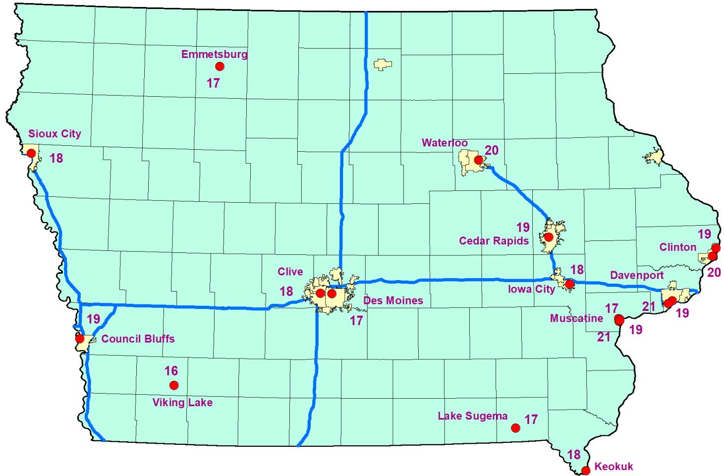
2016-2018 PM 2.5 24-hr Design Values (μg/m 3 )
