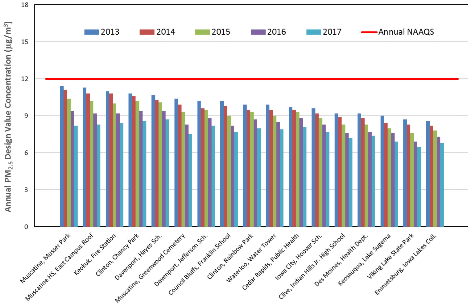
Figure X.2. PM 2.5 Annual Design Values 2013-2017. All Design Values are less than the Annual NAAQS of 12.0 µg/m 3 .
