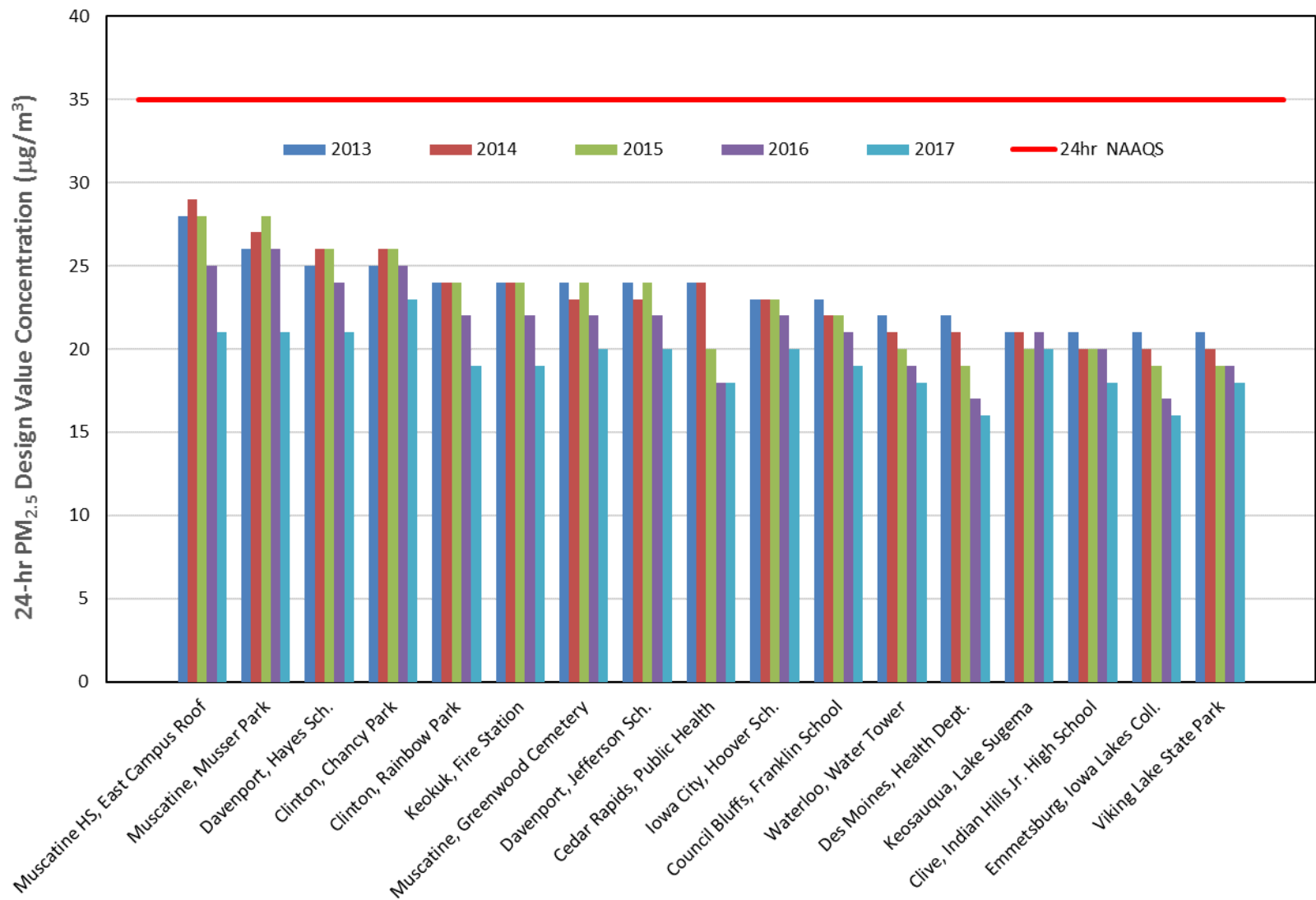
Figure X.1. PM 2.5 24-hr Design Values 2013-2017. All Design Values are less than the 24-hr NAAQS of 35 µg/m 3 .
