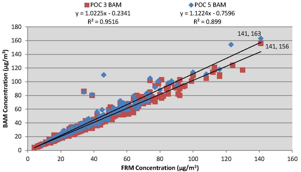
Figure 1. Buffalo, Linnwood Mining PM 10 BAM vs FRM in 2013. For the two points indicated, each BAM records a NAAQS exceedance, while the FRM does not.
