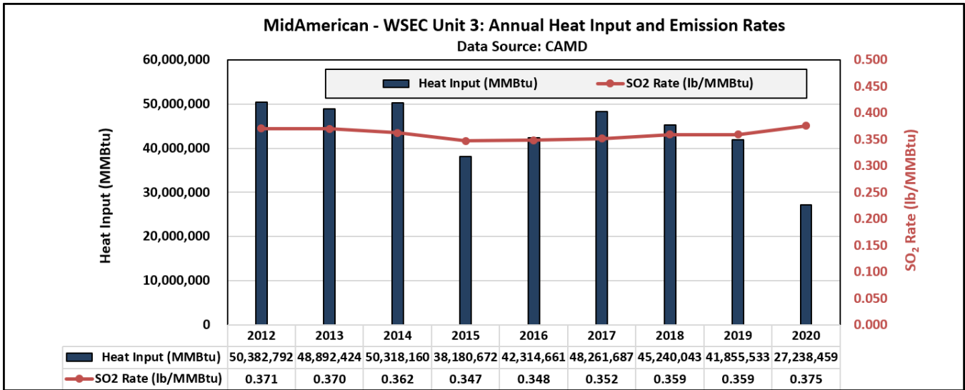
Figure 3-3. Annual 2012-2020 heat input (MMBtu) and SO 2 emission rates (lb/MMBtu) from Unit 3 at WSEC.
