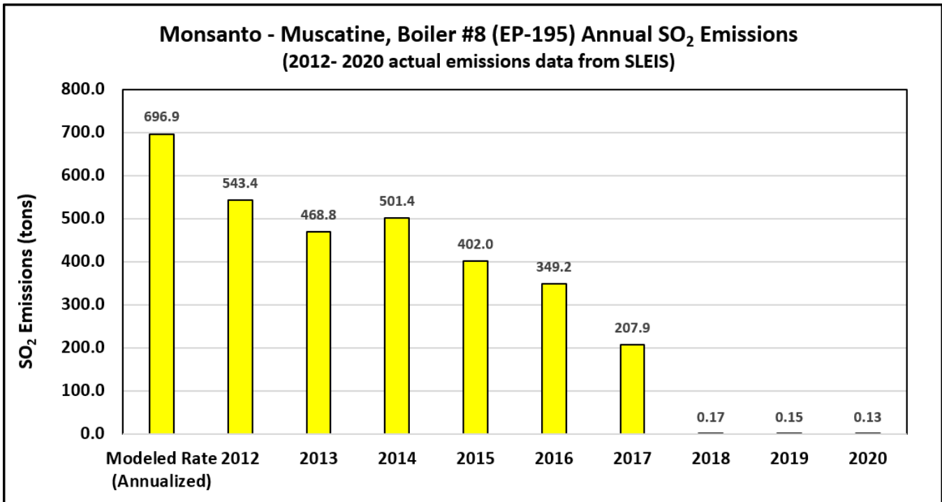
Figure 2-3. Annualized modeled and actual 2012-2020 SO 2 emissions (tons per year) from Boiler #8 at Monsanto. Actual emissions data are from the DNR’s State and Local Emissions Inventory System (SLEIS).
