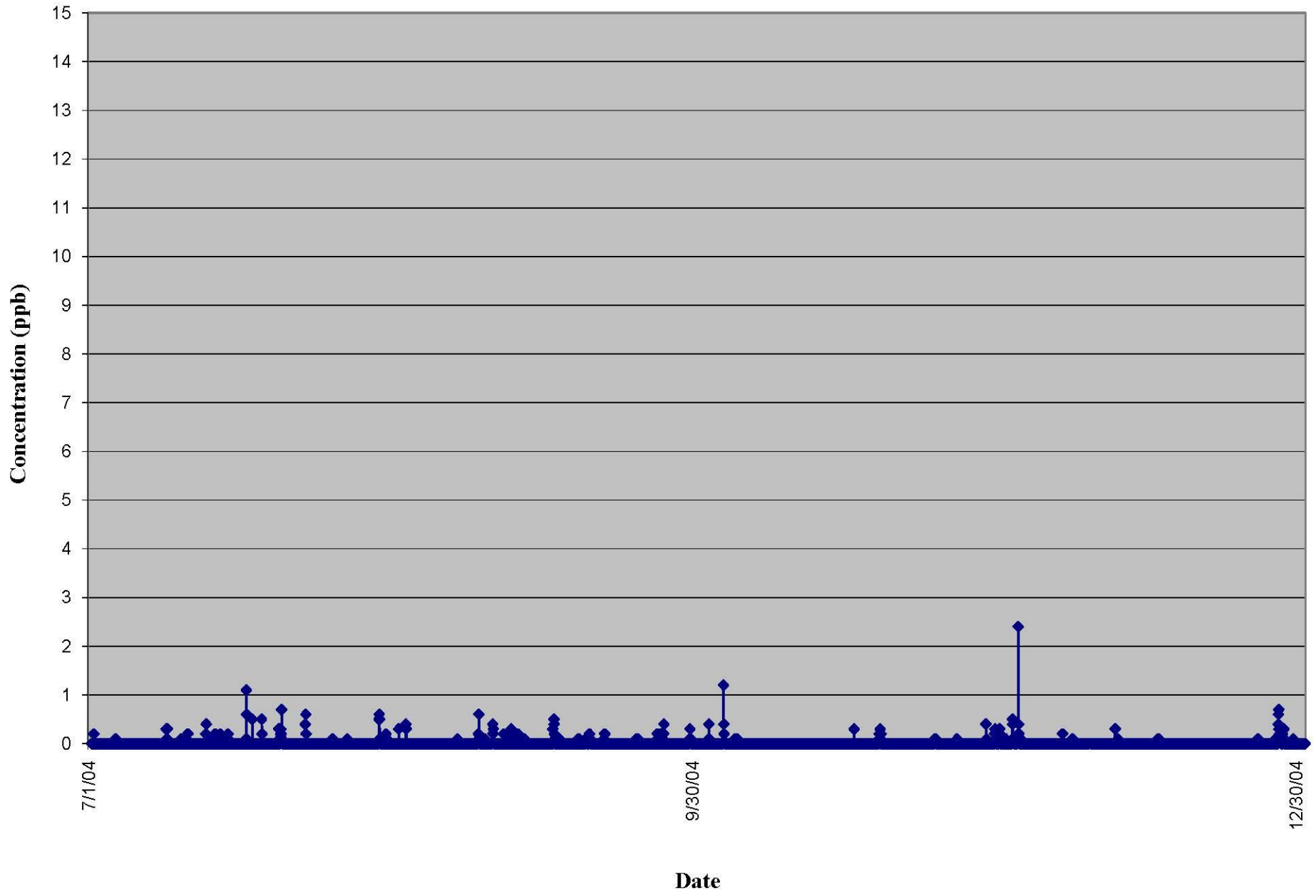
West Union CAFO: Hydrogen Sulfide vs Time (2004)
