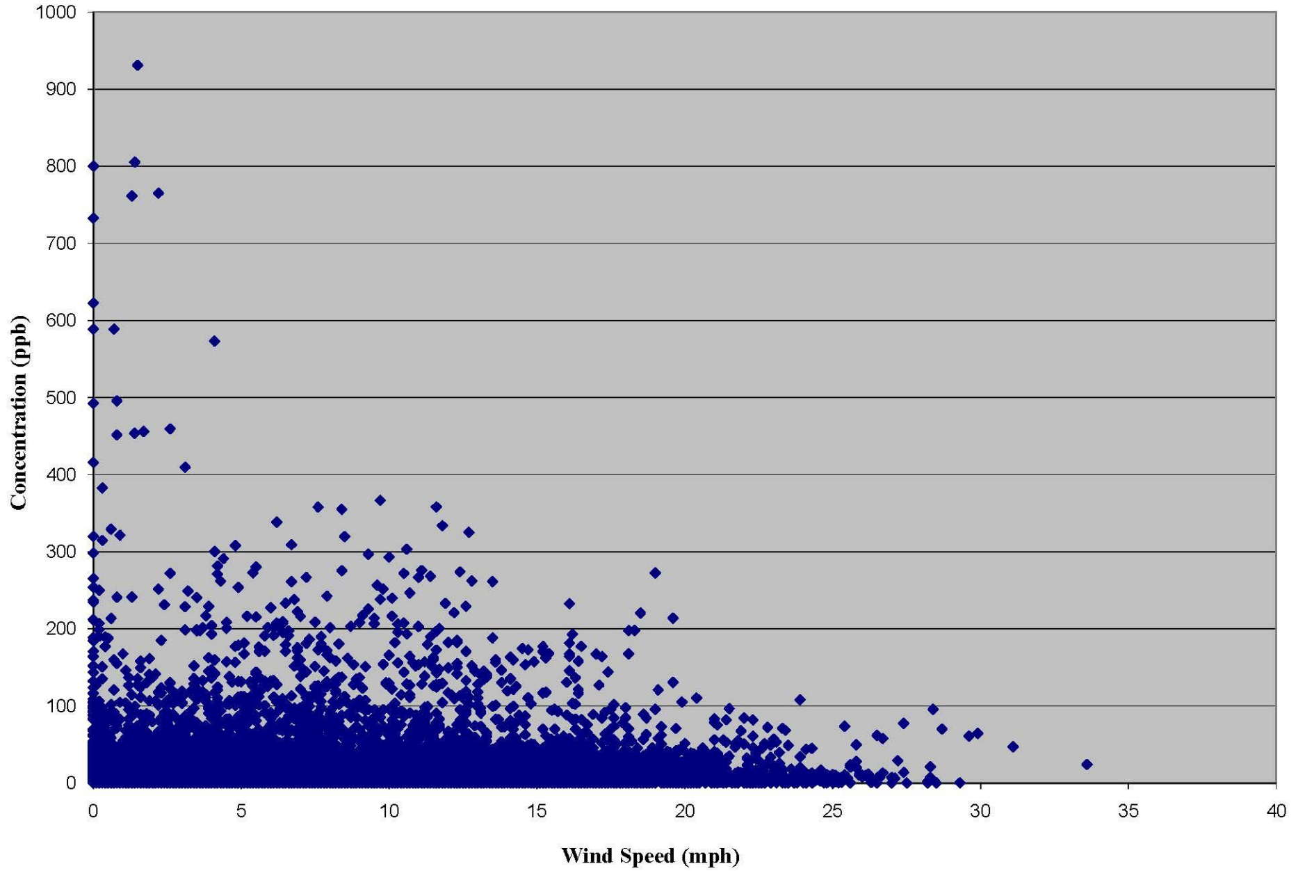
West Union CAFO: Ammonia vs Wind Speed (2004-2007)
