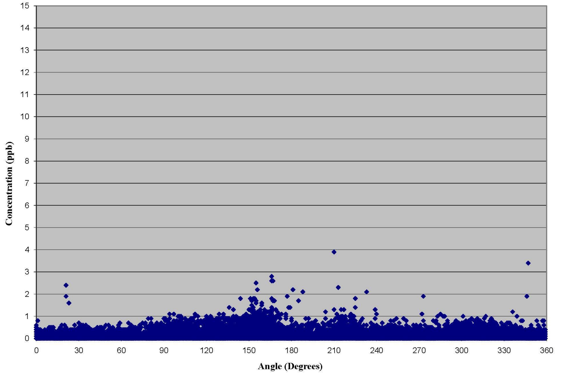
West Union CAFO: Hydrogen Sulfide vs Wind Direction (2004-2007)
