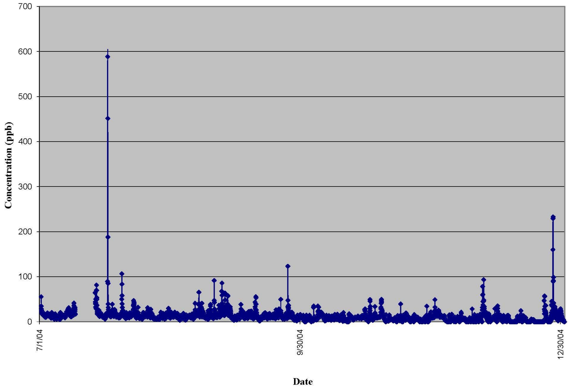
West Union CAFO: Ammonia vs Time (2004)
