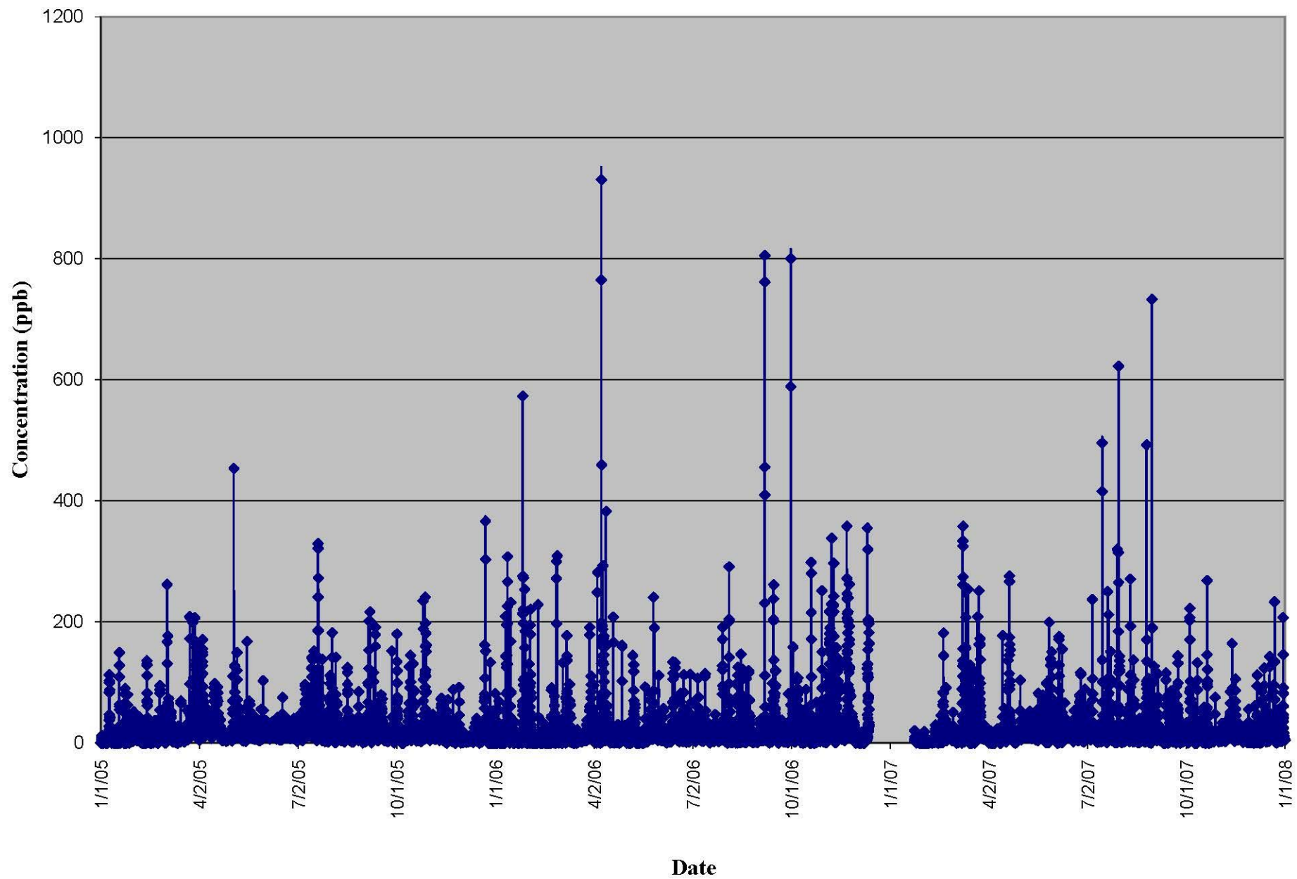
West Union CAFO: Ammonia vs Time (2005-2007)
