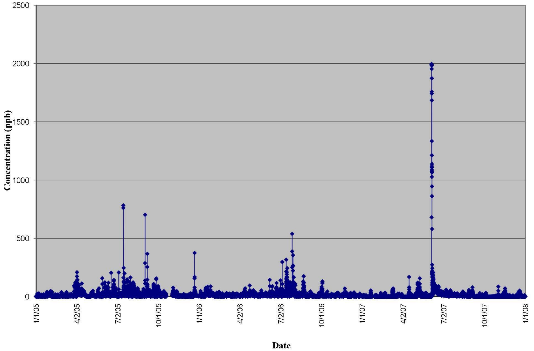
Goldfield CAFO: Ammonia vs Time (2005-2007)
