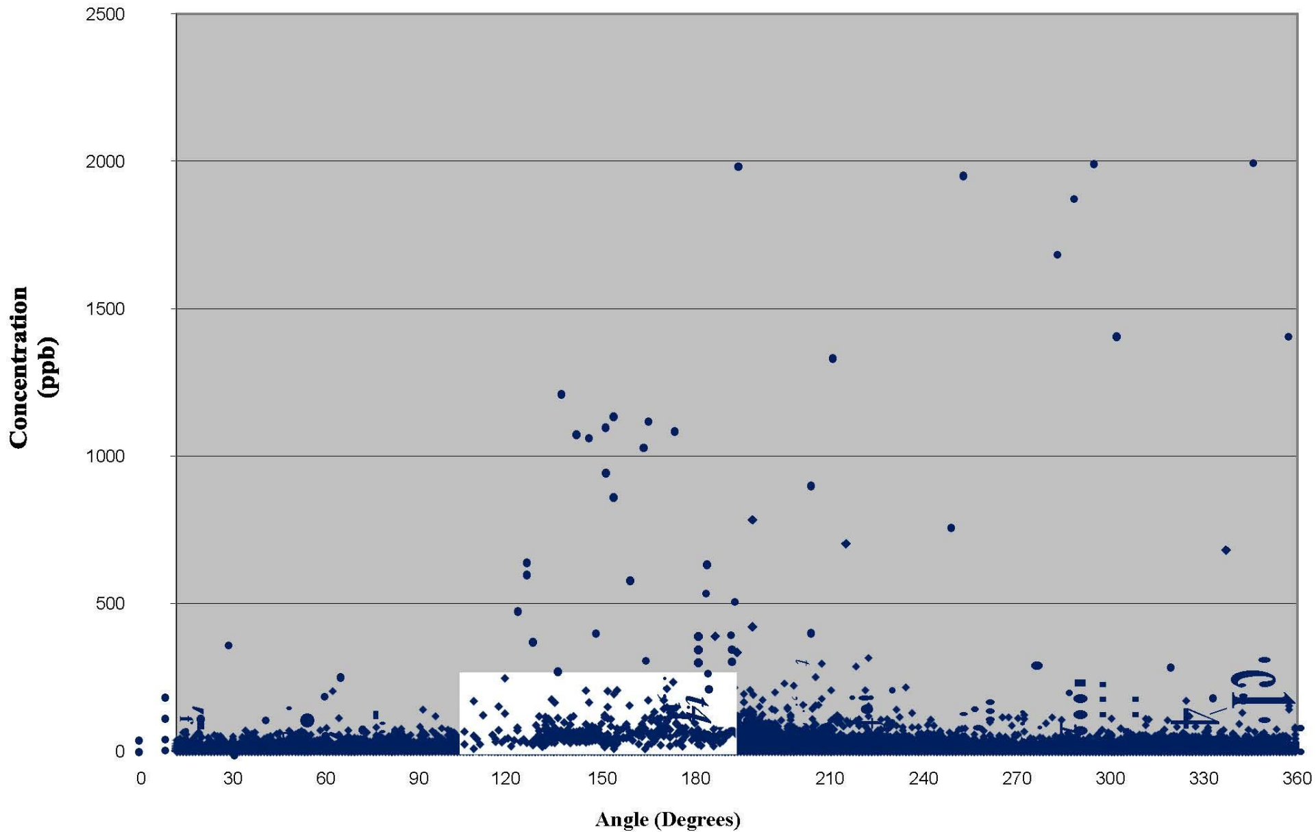
Goldfield CAFO: Ammonia Sulfide vs Wind Direction (2003-2007)
