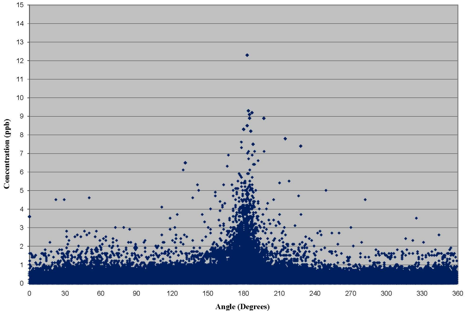
Goldfield CAFO: Hydrogen Sulfide vs Wind Direction (2003-2007)
