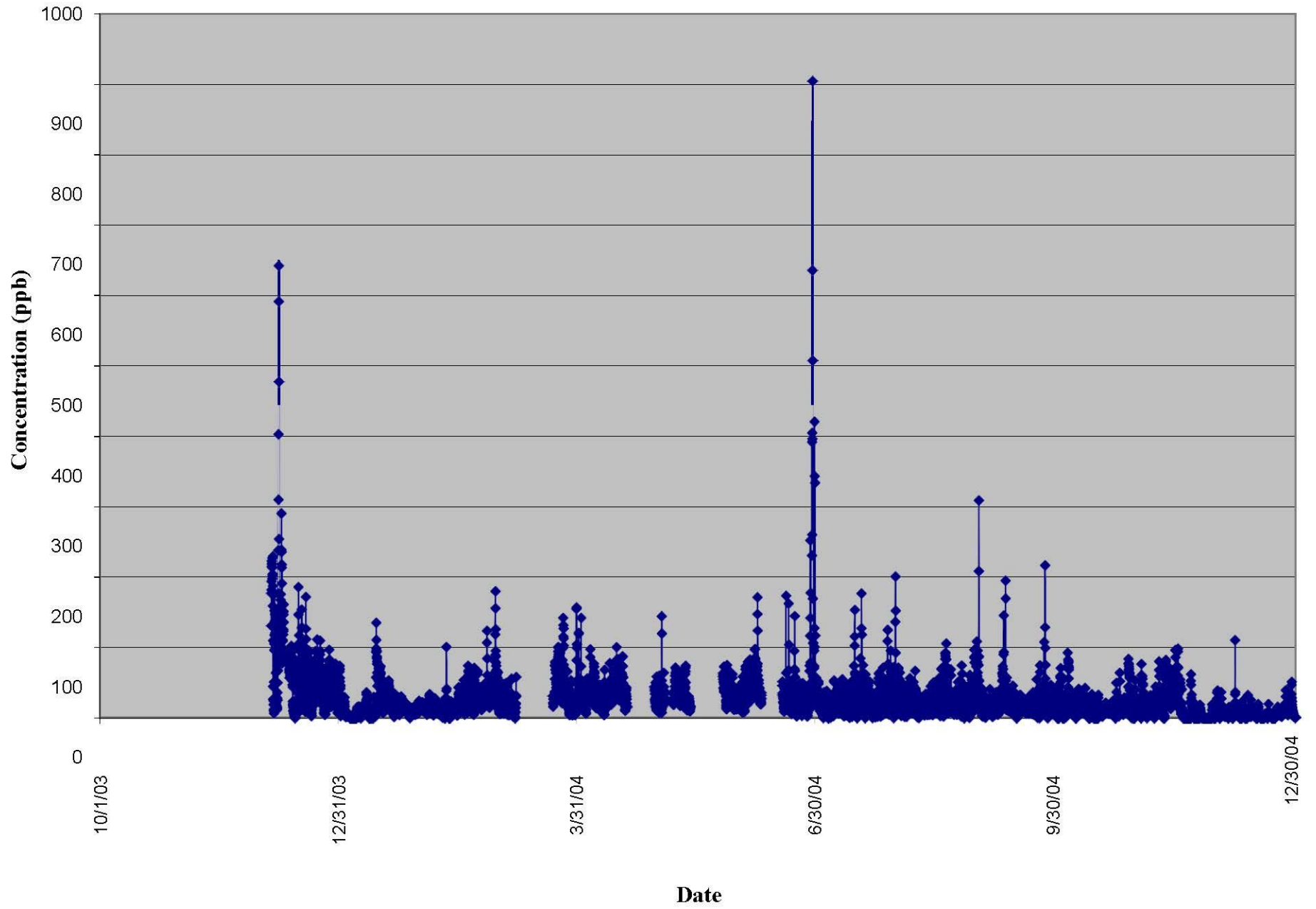
Goldfield CAFO: Ammonia vs Time (2003-2004)
