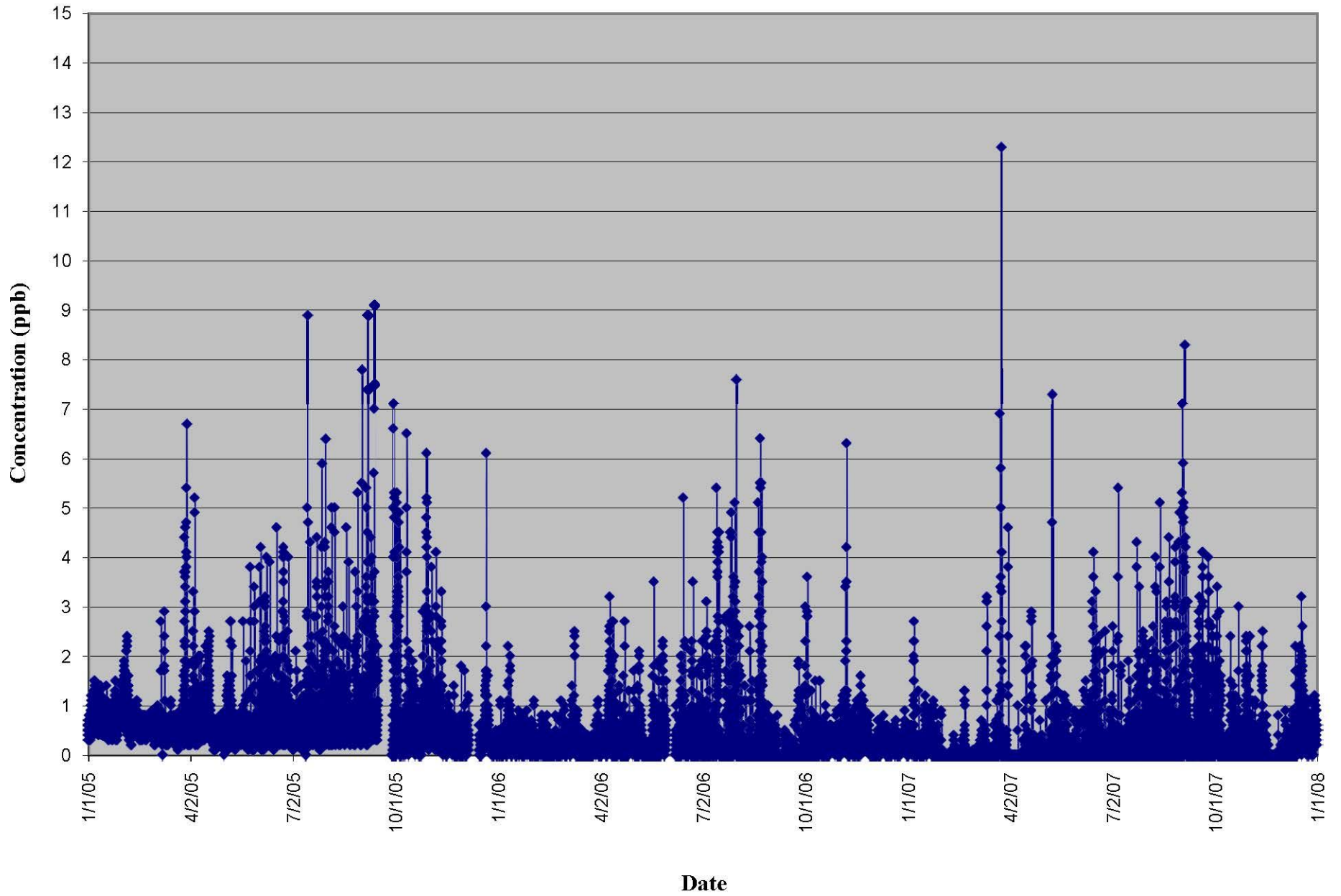
Goldfield CAFO: Hydrogen Sulfide vs Time (2005-2007)
