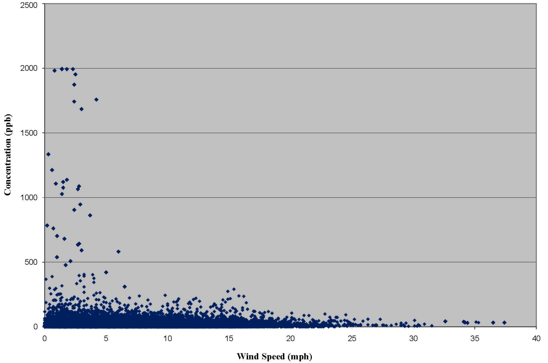
Goldfield CAFO: Ammonia vs Wind Speed (2003-2007)
