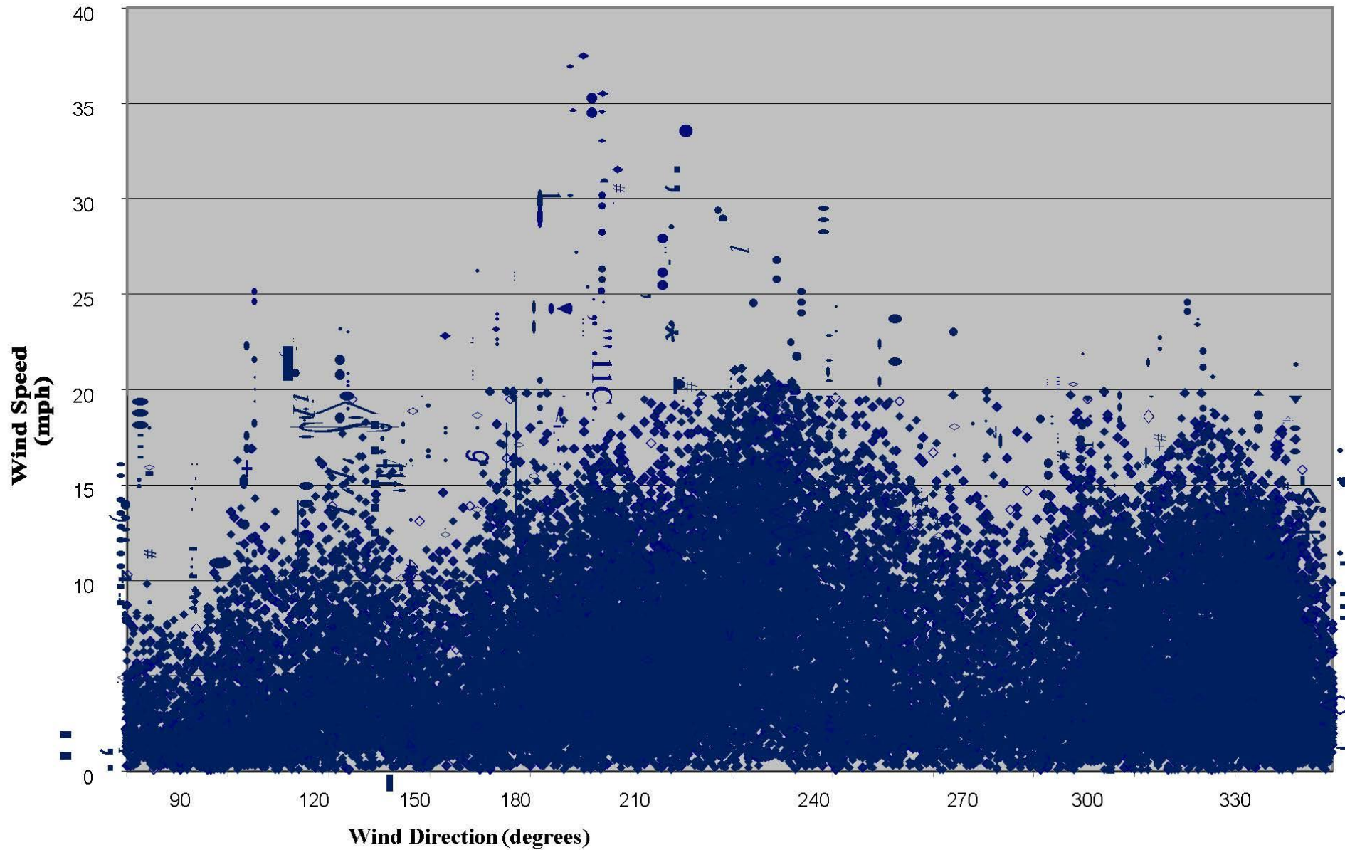
Goldfield CAFO: Wind Speed vs Wind Direction (2003-2007)
