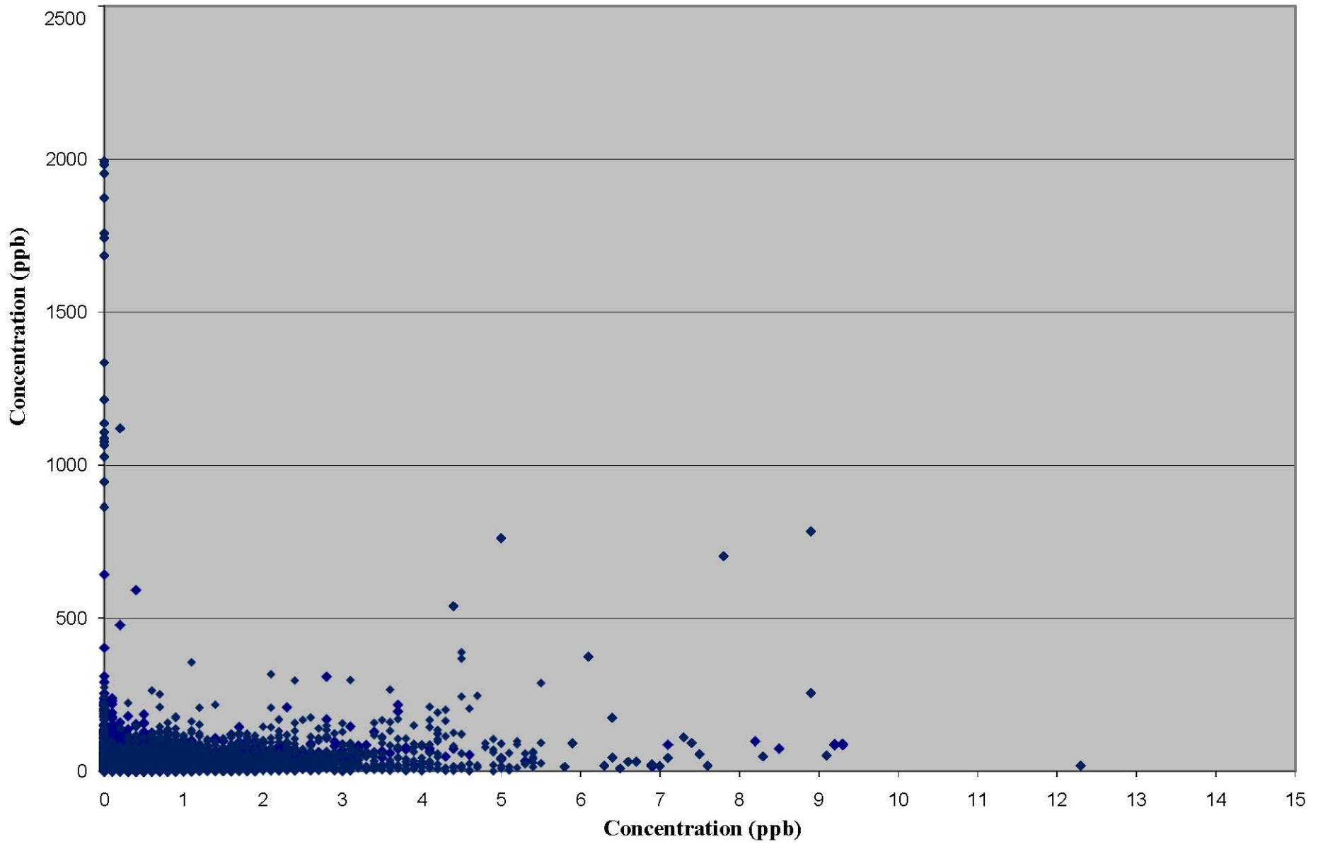
Goldfield CAFO: Ammonia vs Hydrogen Sulfide (2003-2007)
