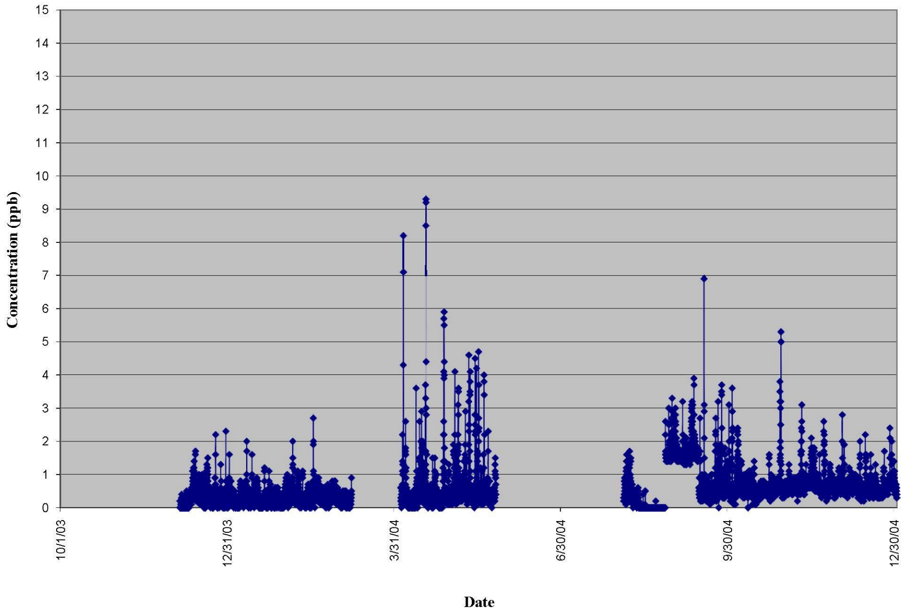
Goldfield CAFO: Hydrogen Sulfide vs Time (2003-2004)
