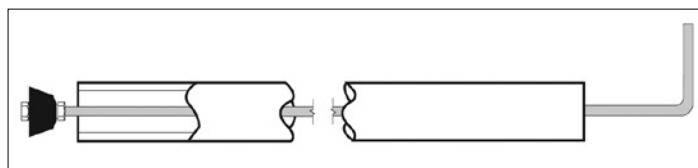
Figure 2. Example sampling probe schematic. Rubber stopper attached to a metal rod to serve as a stopper for PVC manure sampling tube.
